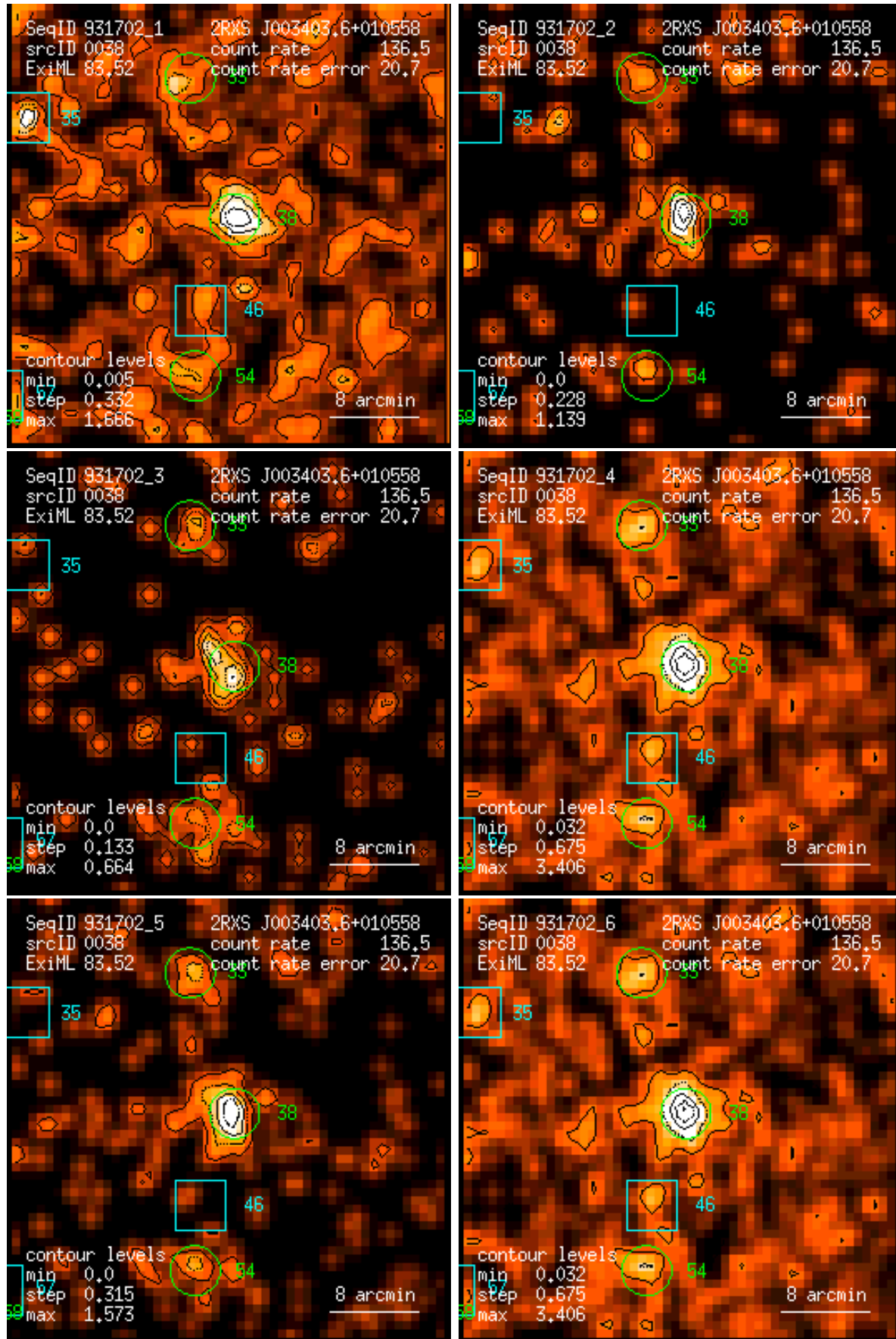
Figure 38: RASS 931702: detection 0038: band rate images, Gaussian filter: (1) PSPC channels 11 – 41, (2) 52 – 90, (3) 91 – 201, (4) 11 – 235, (5) 52 – 201, (6) 11 – 201. Broad band rates in counts/ks. Band rate contour levels in counts/ks/arcmin 2 .
