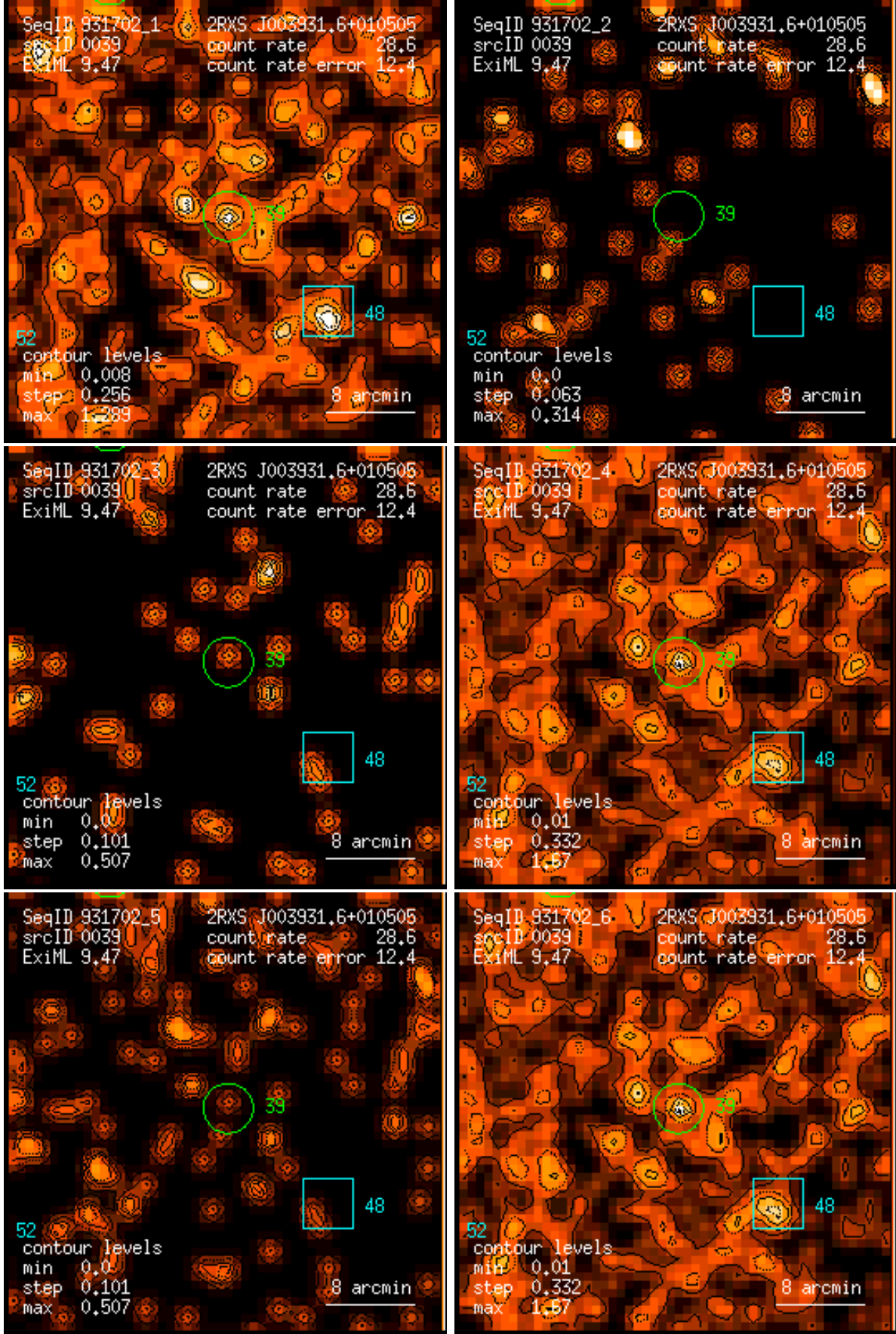
Figure 39: RASS 931702: detection 0039: band rate images, Gaussian filter: (1) PSPC channels 11 – 41, (2) 52 – 90, (3) 91 – 201, (4) 11 – 235, (5) 52 – 201, (6) 11 – 201. Broad band rates in counts/ks. Band rate contour levels in counts/ks/arcmin 2 .
