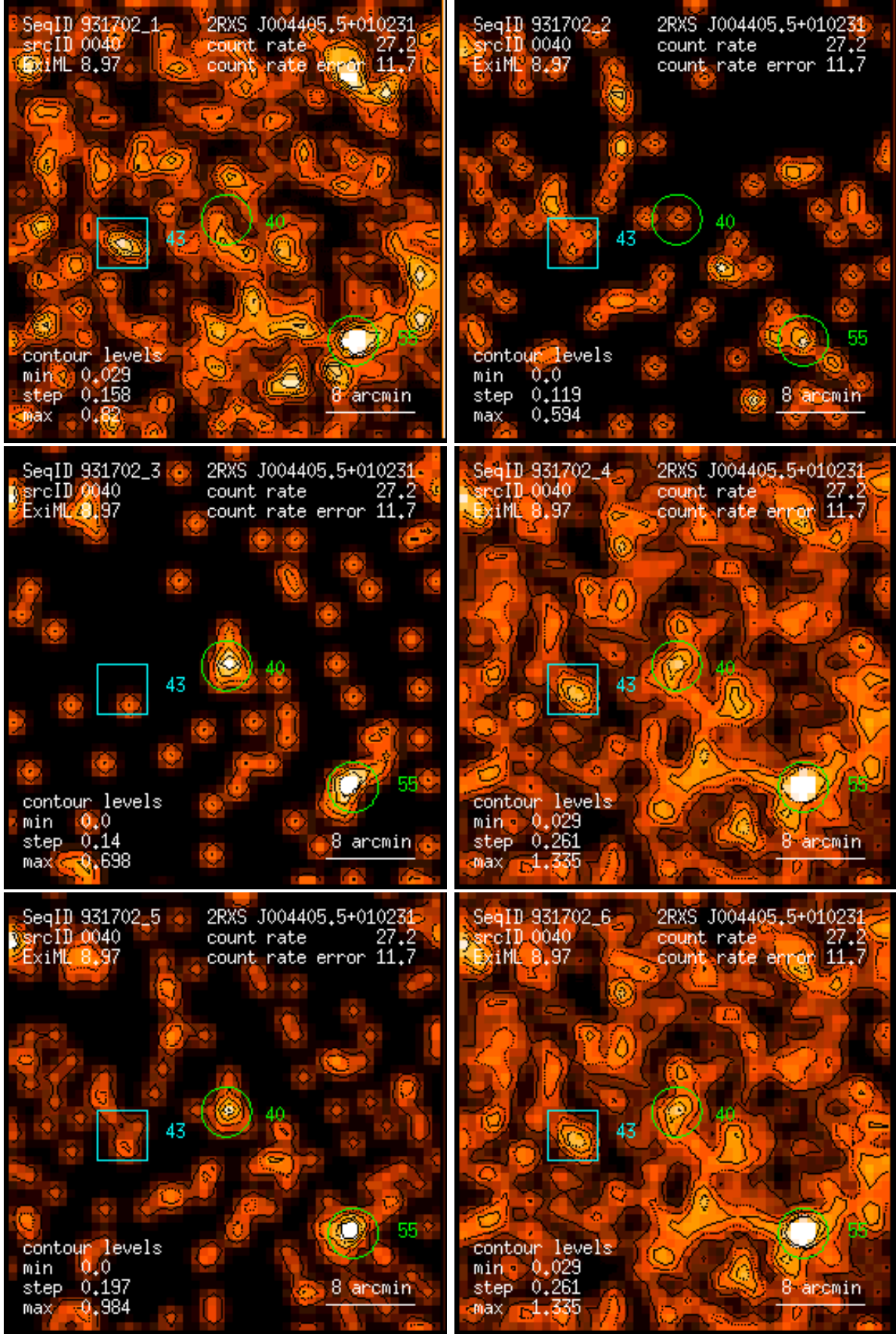
Figure 40: RASS 931702: detection 0040: band rate images, Gaussian filter: (1) PSPC channels 11 – 41, (2) 52 – 90, (3) 91 – 201, (4) 11 – 235, (5) 52 – 201, (6) 11 – 201. Broad band rates in counts/ks. Band rate contour levels in counts/ks/arcmin 2 .
