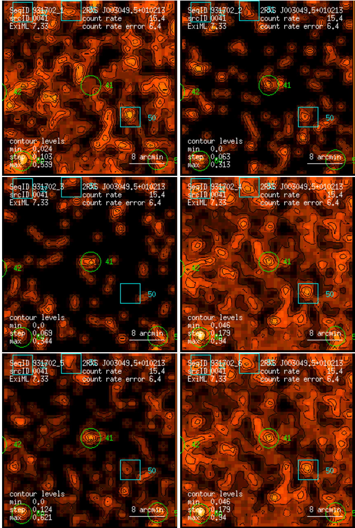
Figure 41: RASS 931702: detection 0041: band rate images, Gaussian filter: (1) PSPC channels 11 – 41, (2) 52 – 90, (3) 91 – 201, (4) 11 – 235, (5) 52 – 201, (6) 11 – 201. Broad band rates in counts/ks. Band rate contour levels in counts/ks/arcmin 2 .
