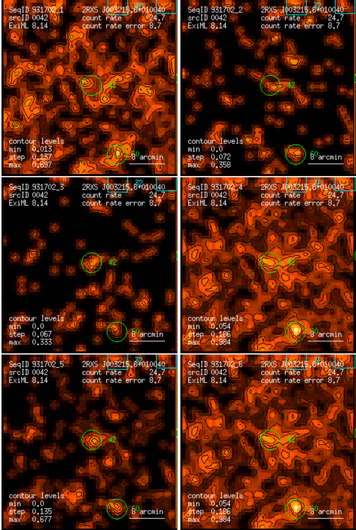
Figure 42: RASS 931702: detection 0042: band rate images, Gaussian filter: (1) PSPC channels 11 – 41, (2) 52 – 90, (3) 91 – 201, (4) 11 – 235, (5) 52 – 201, (6) 11 – 201. Broad band rates in counts/ks. Band rate contour levels in counts/ks/arcmin 2 .
