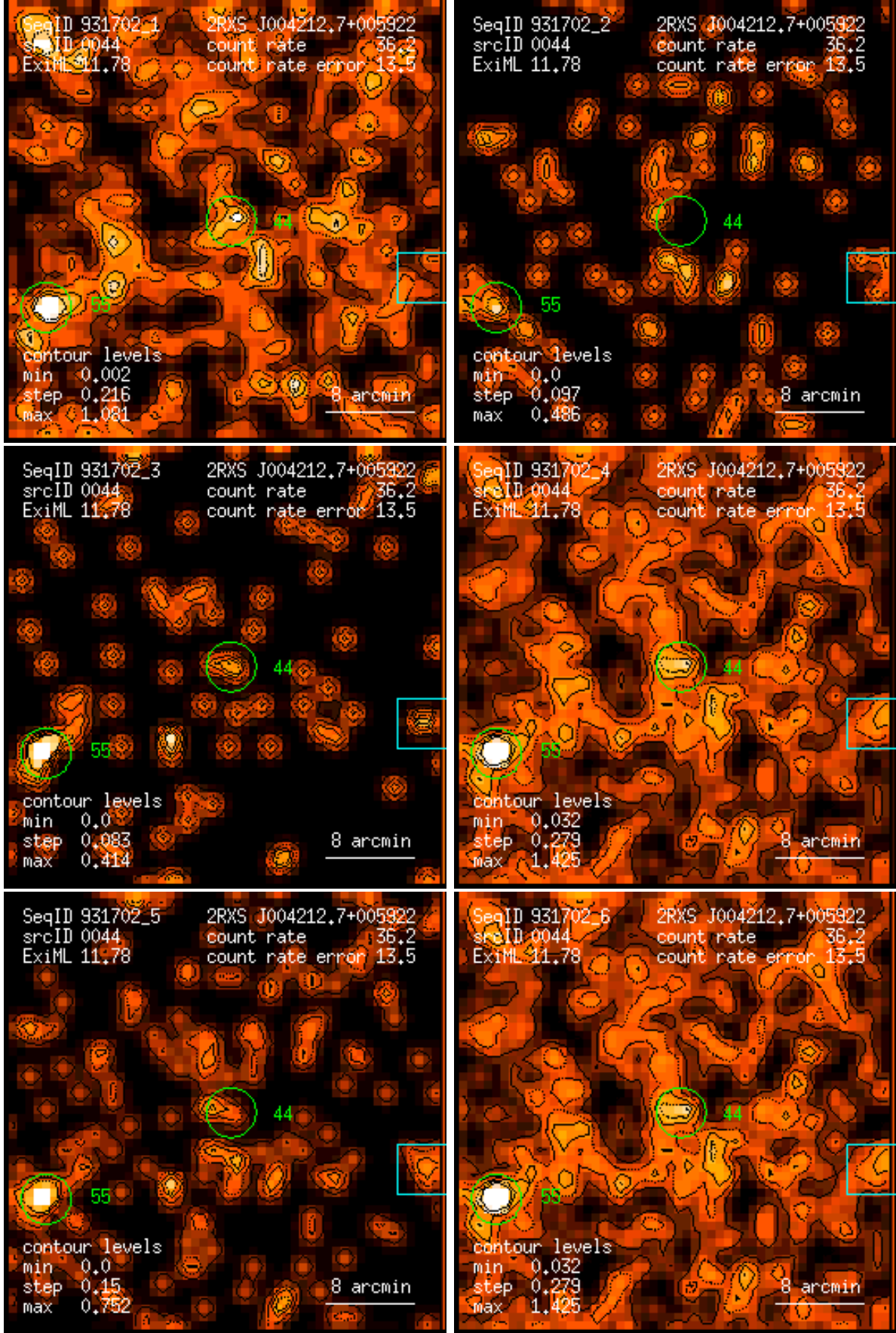
Figure 44: RASS 931702: detection 0044: band rate images, Gaussian filter: (1) PSPC channels 11 – 41, (2) 52 – 90, (3) 91 – 201, (4) 11 – 235, (5) 52 – 201, (6) 11 – 201. Broad band rates in counts/ks. Band rate contour levels in counts/ks/arcmin 2 .
