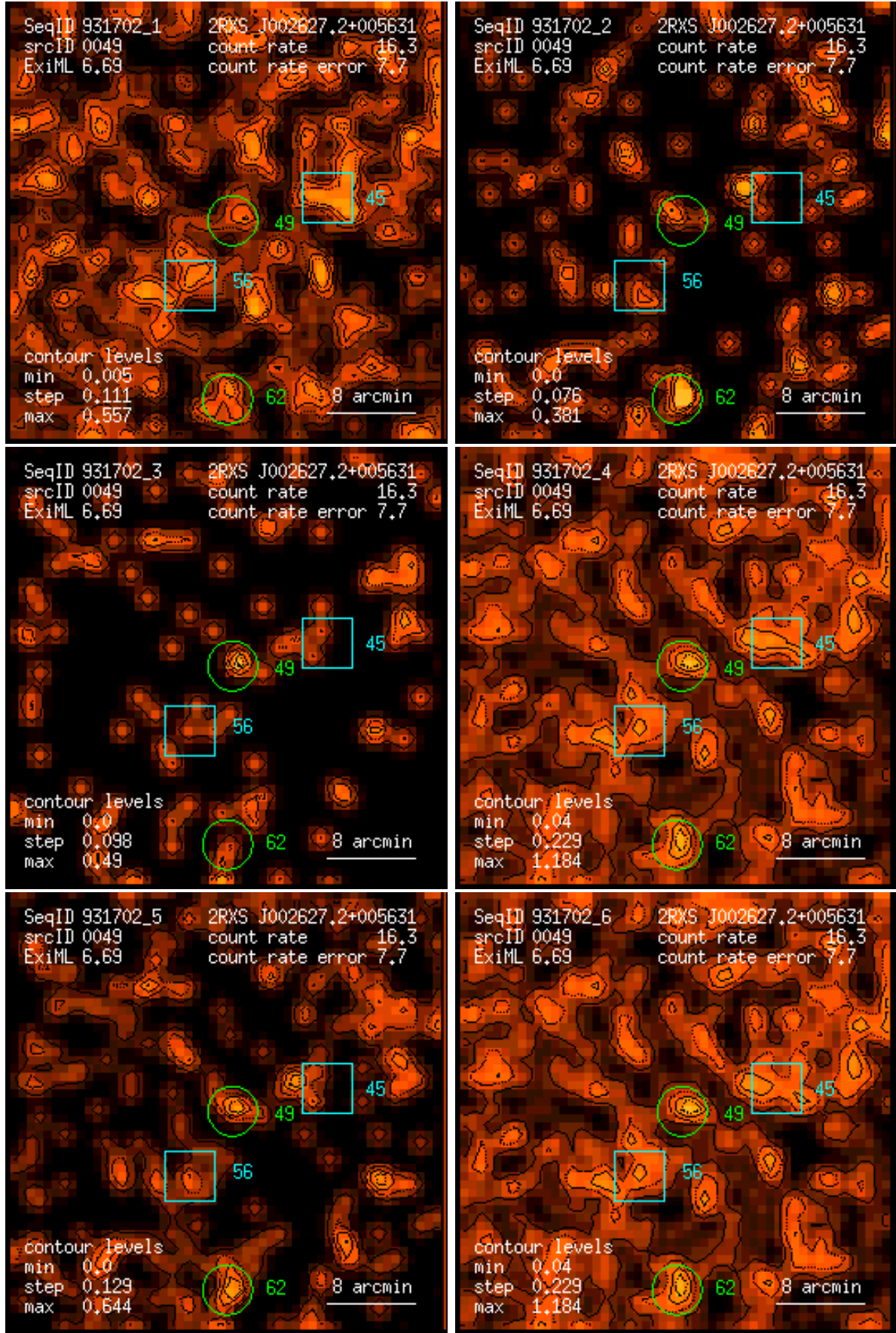
Figure 49: RASS 931702: detection 0049: band rate images, Gaussian filter: (1) PSPC channels 11 – 41, (2) 52 – 90, (3) 91 – 201, (4) 11 – 235, (5) 52 – 201, (6) 11 – 201. Broad band rates in counts/ks. Band rate contour levels in counts/ks/arcmin 2 .
