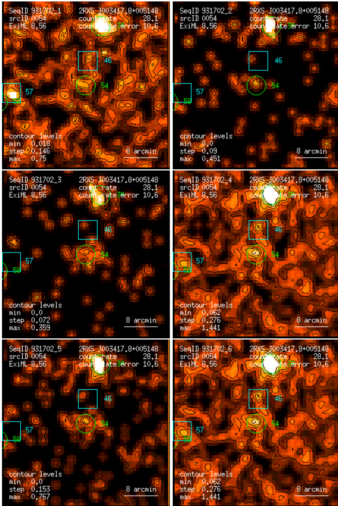
Figure 54: RASS 931702: detection 0054: band rate images, Gaussian filter: (1) PSPC channels 11 – 41, (2) 52 – 90, (3) 91 – 201, (4) 11 – 235, (5) 52 – 201, (6) 11 – 201. Broad band rates in counts/ks. Band rate contour levels in counts/ks/arcmin 2 .
