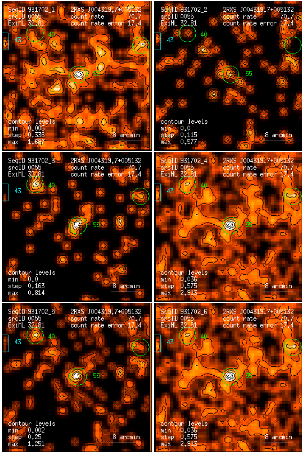
Figure 55: RASS 931702: detection 0055: band rate images, Gaussian filter: (1) PSPC channels 11 – 41, (2) 52 – 90, (3) 91 – 201, (4) 11 – 235, (5) 52 – 201, (6) 11 – 201. Broad band rates in counts/ks. Band rate contour levels in counts/ks/arcmin 2 .
