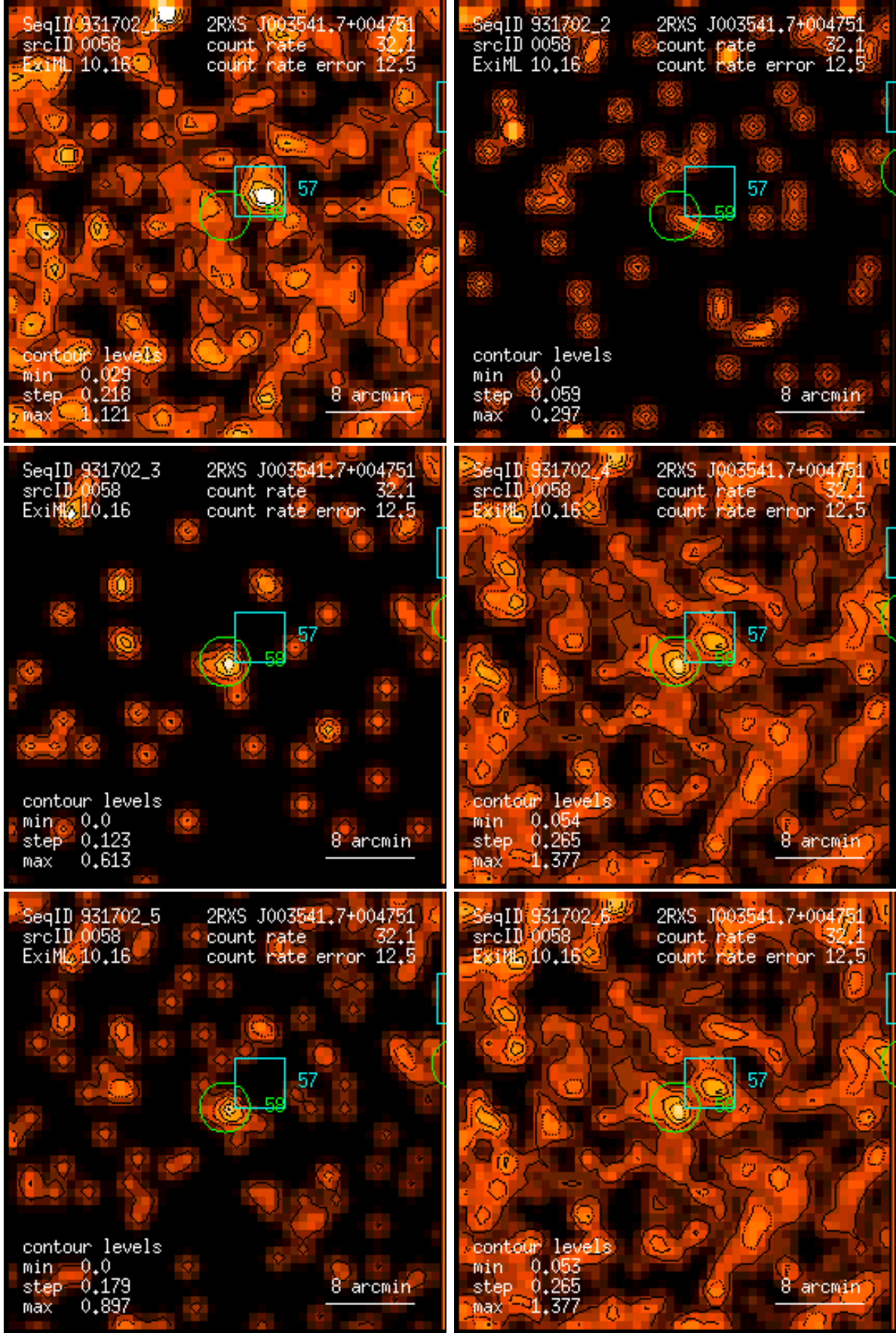
Figure 58: RASS 931702: detection 0058: band rate images, Gaussian filter: (1) PSPC channels 11 – 41, (2) 52 – 90, (3) 91 – 201, (4) 11 – 235, (5) 52 – 201, (6) 11 – 201. Broad band rates in counts/ks. Band rate contour levels in counts/ks/arcmin 2 .
