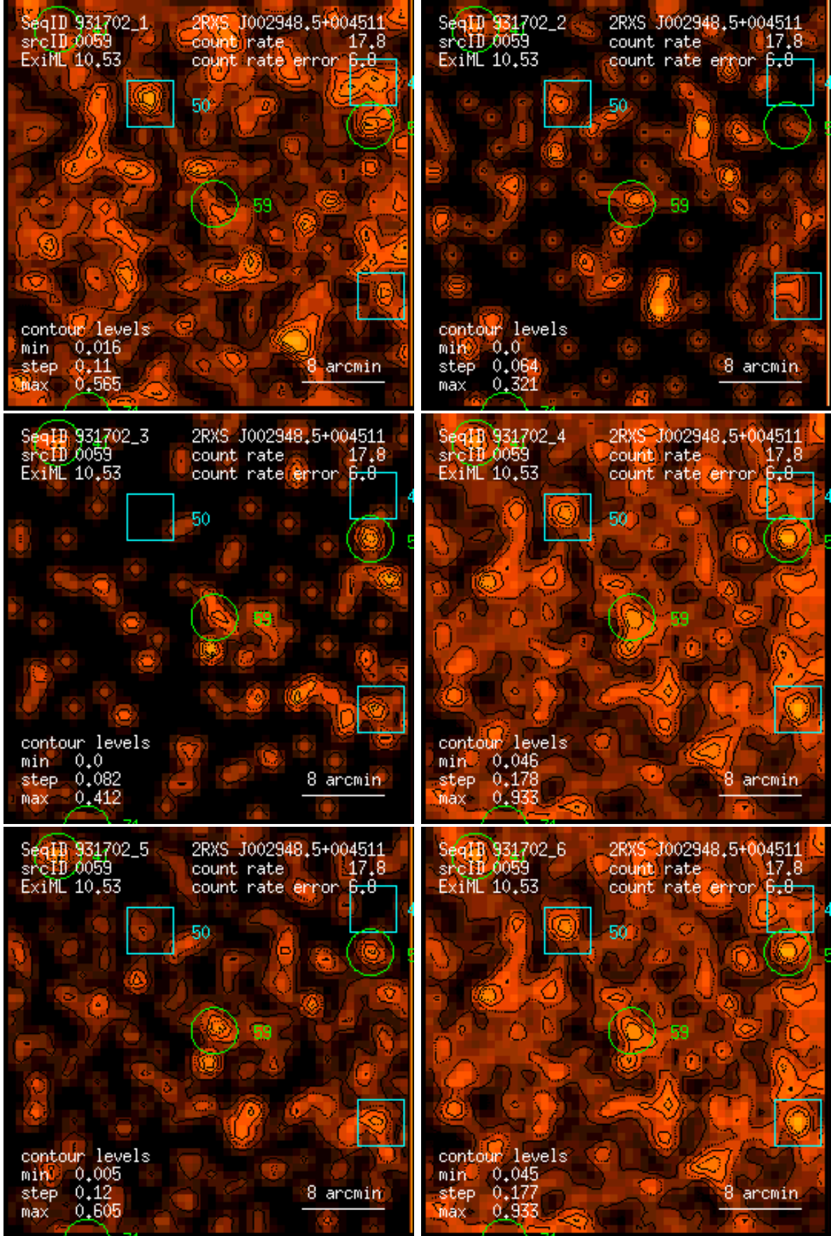
Figure 59: RASS 931702: detection 0059: band rate images, Gaussian filter: (1) PSPC channels 11 – 41, (2) 52 – 90, (3) 91 – 201, (4) 11 – 235, (5) 52 – 201, (6) 11 – 201. Broad band rates in counts/ks. Band rate contour levels in counts/ks/arcmin 2 .
