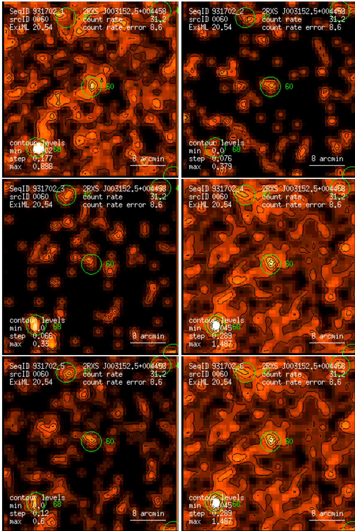
Figure 60: RASS 931702: detection 0060: band rate images, Gaussian filter: (1) PSPC channels 11 – 41, (2) 52 – 90, (3) 91 – 201, (4) 11 – 235, (5) 52 – 201, (6) 11 – 201. Broad band rates in counts/ks. Band rate contour levels in counts/ks/arcmin 2 .
