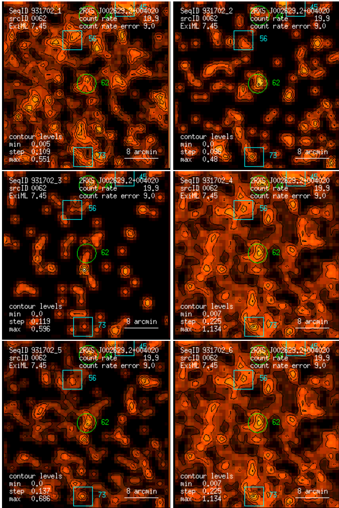
Figure 62: RASS 931702: detection 0062: band rate images, Gaussian filter: (1) PSPC channels 11 – 41, (2) 52 – 90, (3) 91 – 201, (4) 11 – 235, (5) 52 – 201, (6) 11 – 201. Broad band rates in counts/ks. Band rate contour levels in counts/ks/arcmin 2 .
