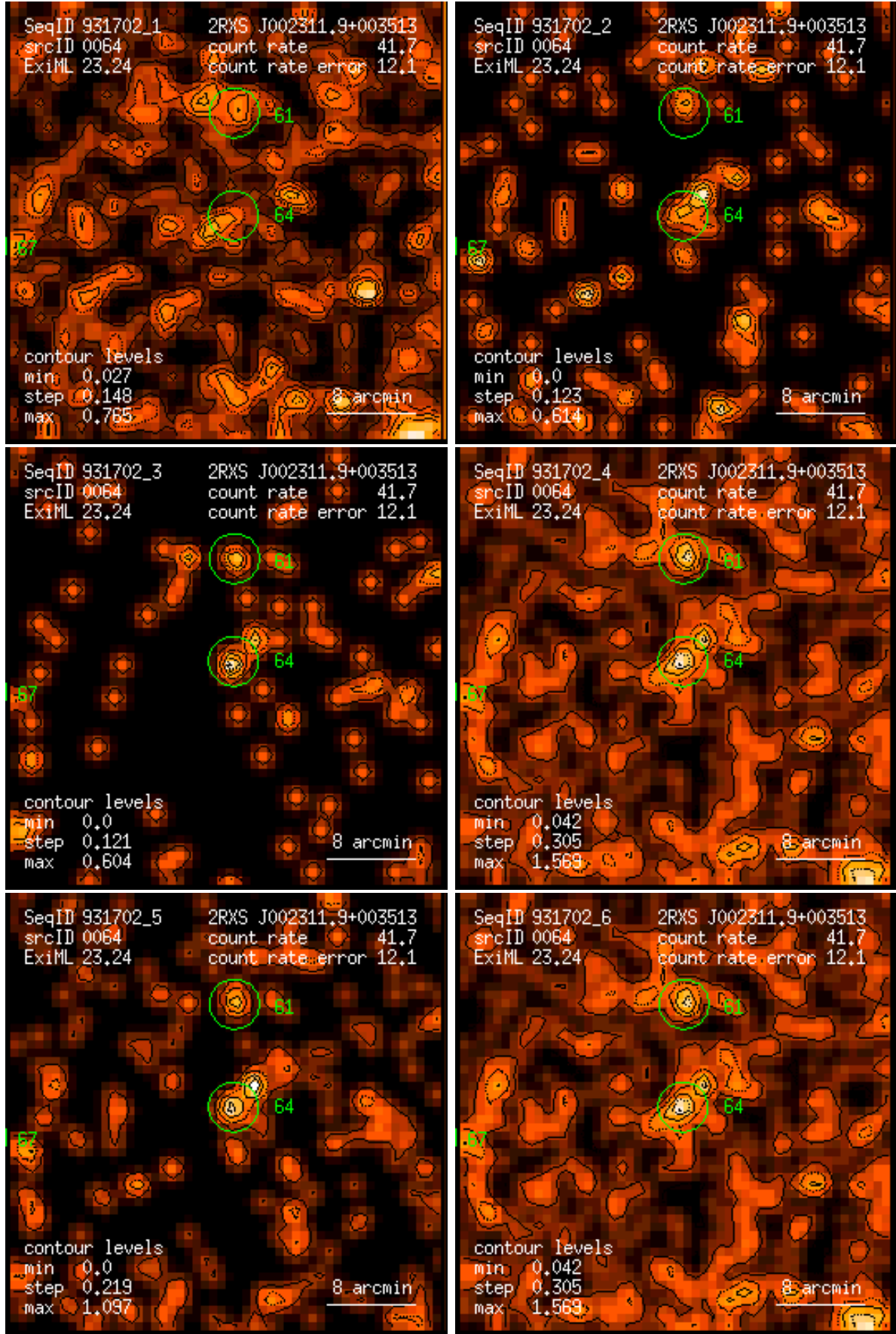
Figure 64: RASS 931702: detection 0064: band rate images, Gaussian filter: (1) PSPC channels 11 – 41, (2) 52 – 90, (3) 91 – 201, (4) 11 – 235, (5) 52 – 201, (6) 11 – 201. Broad band rates in counts/ks. Band rate contour levels in counts/ks/arcmin 2 .
