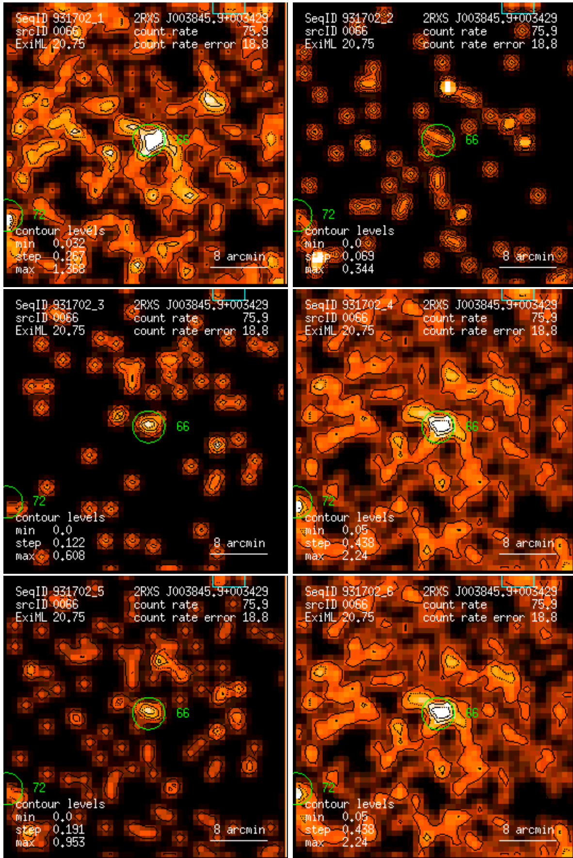
Figure 66: RASS 931702: detection 0066: band rate images, Gaussian filter: (1) PSPC channels 11 – 41, (2) 52 – 90, (3) 91 – 201, (4) 11 – 235, (5) 52 – 201, (6) 11 – 201. Broad band rates in counts/ks. Band rate contour levels in counts/ks/arcmin 2 .
