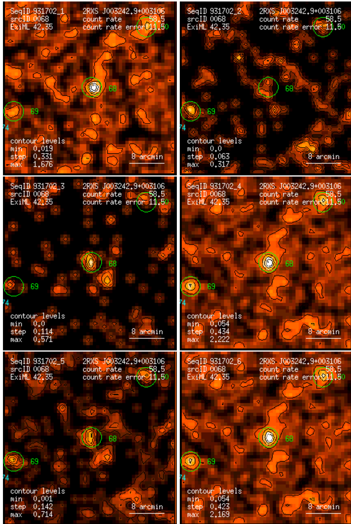
Figure 68: RASS 931702: detection 0068: band rate images, Gaussian filter: (1) PSPC channels 11 – 41, (2) 52 – 90, (3) 91 – 201, (4) 11 – 235, (5) 52 – 201, (6) 11 – 201. Broad band rates in counts/ks. Band rate contour levels in counts/ks/arcmin 2 .
