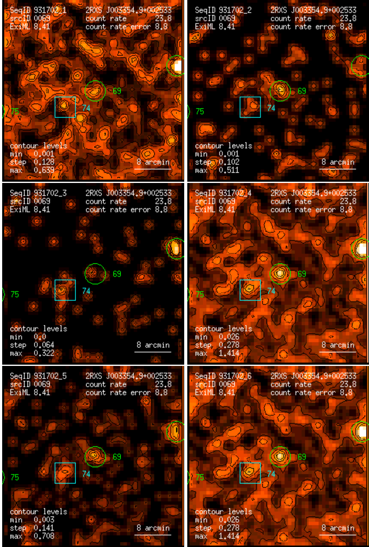
Figure 69: RASS 931702: detection 0069: band rate images, Gaussian filter: (1) PSPC channels 11 – 41, (2) 52 – 90, (3) 91 – 201, (4) 11 – 235, (5) 52 – 201, (6) 11 – 201. Broad band rates in counts/ks. Band rate contour levels in counts/ks/arcmin 2 .
