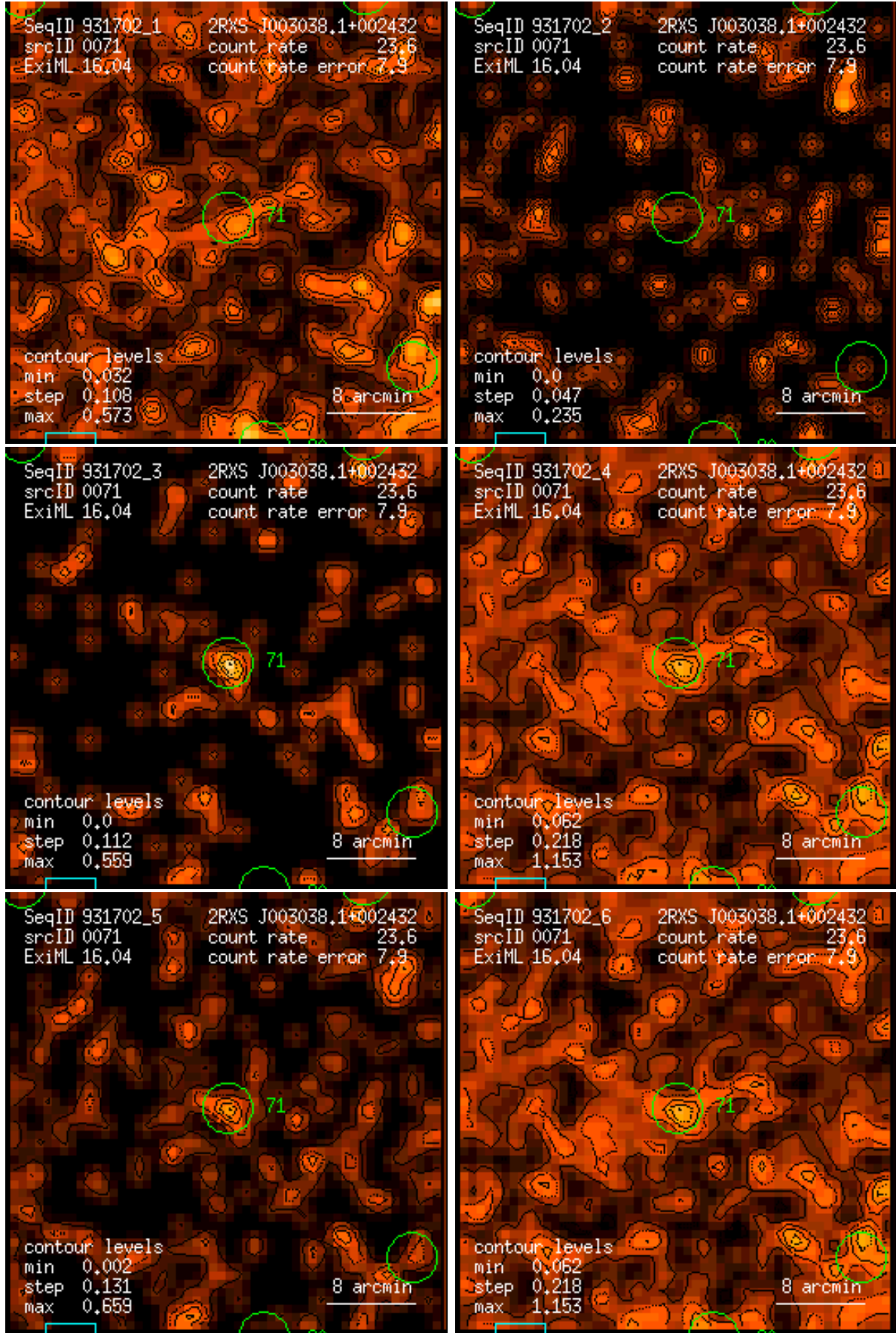
Figure 71: RASS 931702: detection 0071: band rate images, Gaussian filter: (1) PSPC channels 11 – 41, (2) 52 – 90, (3) 91 – 201, (4) 11 – 235, (5) 52 – 201, (6) 11 – 201. Broad band rates in counts/ks. Band rate contour levels in counts/ks/arcmin 2 .
