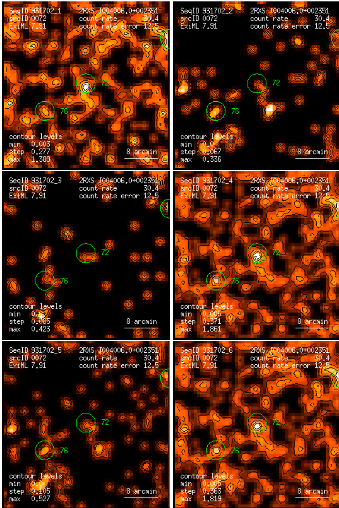
Figure 72: RASS 931702: detection 0072: band rate images, Gaussian filter: (1) PSPC channels 11 – 41, (2) 52 – 90, (3) 91 – 201, (4) 11 – 235, (5) 52 – 201, (6) 11 – 201. Broad band rates in counts/ks. Band rate contour levels in counts/ks/arcmin 2 .
