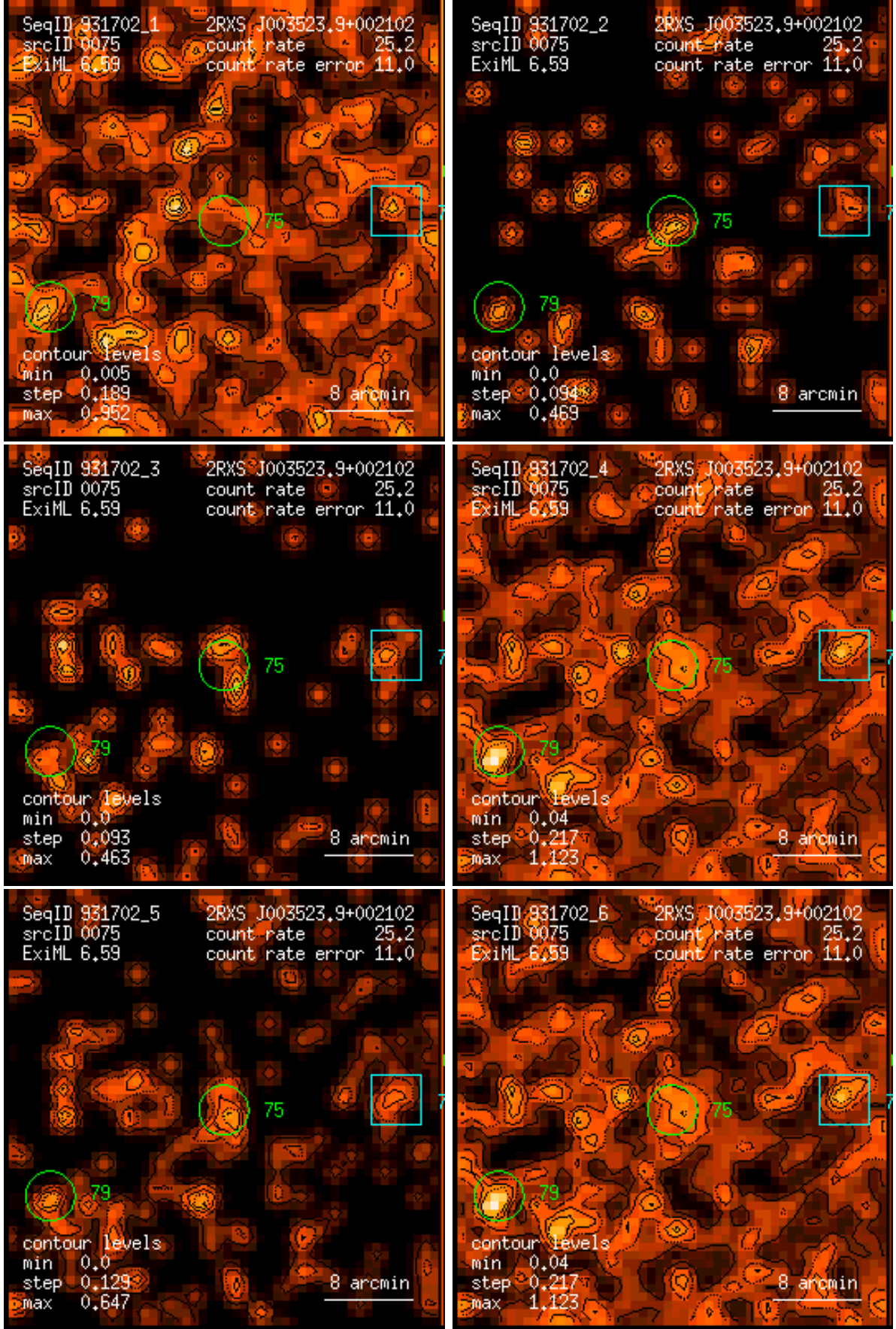
Figure 75: RASS 931702: detection 0075: band rate images, Gaussian filter: (1) PSPC channels 11 – 41, (2) 52 – 90, (3) 91 – 201, (4) 11 – 235, (5) 52 – 201, (6) 11 – 201. Broad band rates in counts/ks. Band rate contour levels in counts/ks/arcmin 2 .
