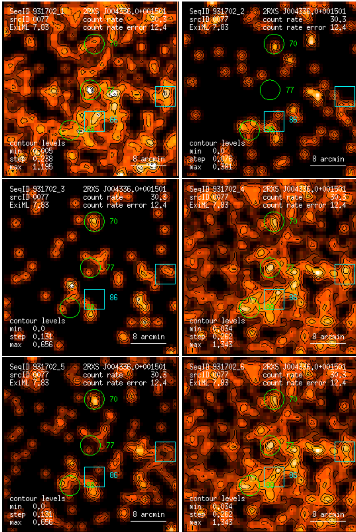
Figure 77: RASS 931702: detection 0077: band rate images, Gaussian filter: (1) PSPC channels 11 – 41, (2) 52 – 90, (3) 91 – 201, (4) 11 – 235, (5) 52 – 201, (6) 11 – 201. Broad band rates in counts/ks. Band rate contour levels in counts/ks/arcmin 2 .
