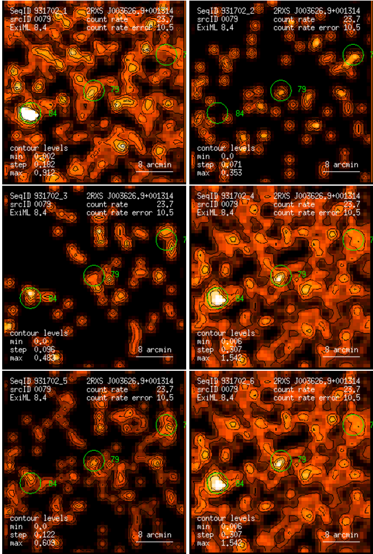
Figure 79: RASS 931702: detection 0079: band rate images, Gaussian filter: (1) PSPC channels 11 – 41, (2) 52 – 90, (3) 91 – 201, (4) 11 – 235, (5) 52 – 201, (6) 11 – 201. Broad band rates in counts/ks. Band rate contour levels in counts/ks/arcmin 2 .
