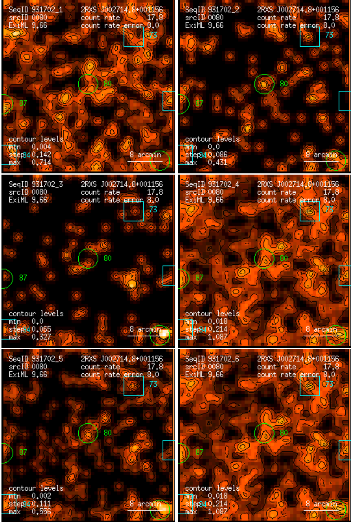
Figure 80: RASS 931702: detection 0080: band rate images, Gaussian filter: (1) PSPC channels 11 – 41, (2) 52 – 90, (3) 91 – 201, (4) 11 – 235, (5) 52 – 201, (6) 11 – 201. Broad band rates in counts/ks. Band rate contour levels in counts/ks/arcmin 2 .
