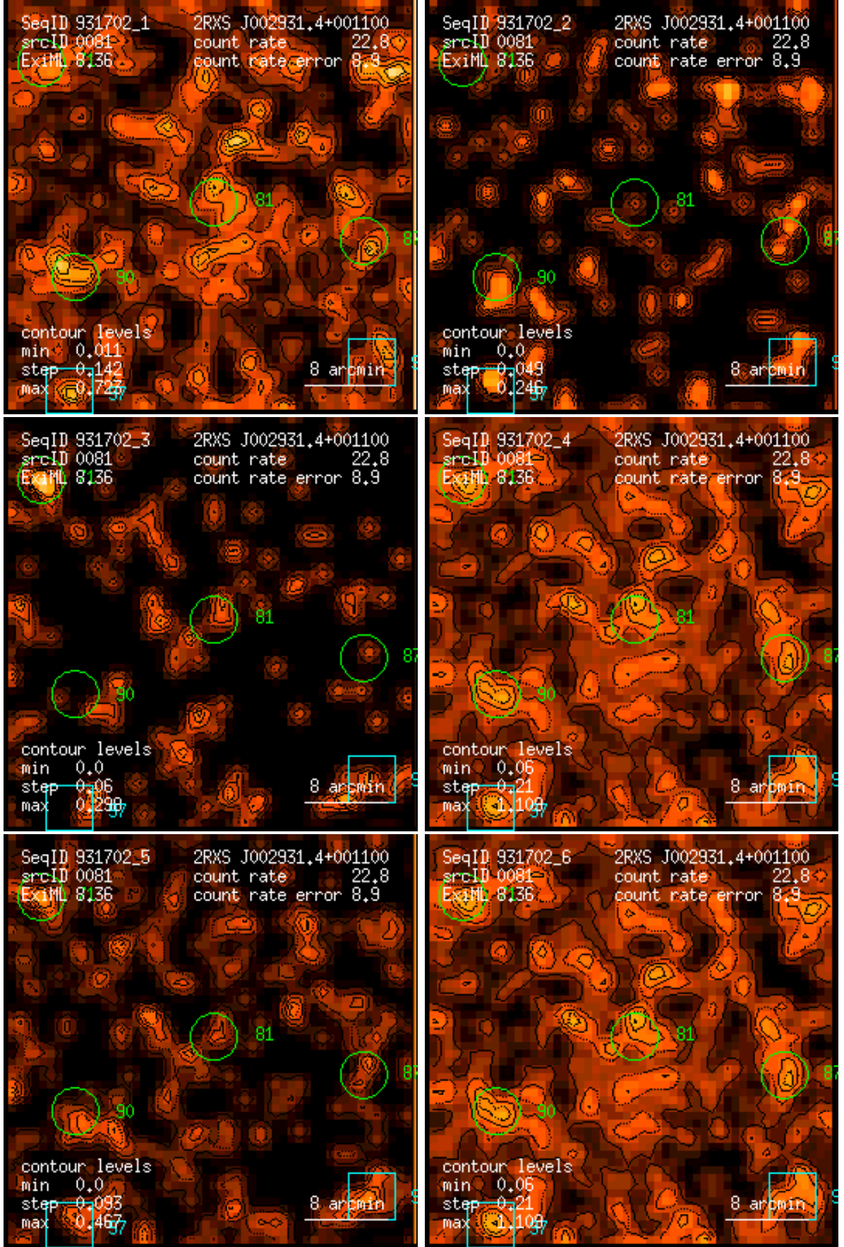
Figure 81: RASS 931702: detection 0081: band rate images, Gaussian filter: (1) PSPC channels 11 – 41, (2) 52 – 90, (3) 91 – 201, (4) 11 – 235, (5) 52 – 201, (6) 11 – 201. Broad band rates in counts/ks. Band rate contour levels in counts/ks/arcmin 2 .
