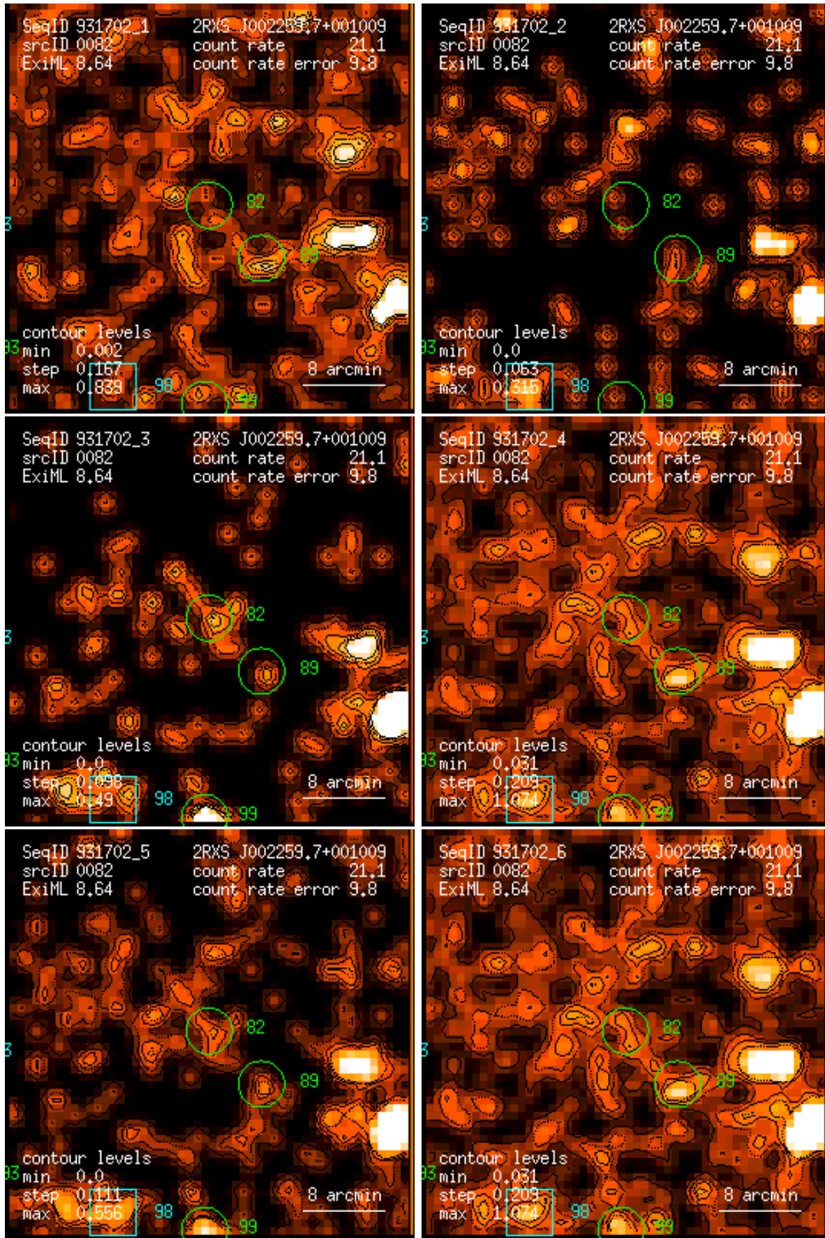
Figure 82: RASS 931702: detection 0082: band rate images, Gaussian filter: (1) PSPC channels 11 – 41, (2) 52 – 90, (3) 91 – 201, (4) 11 – 235, (5) 52 – 201, (6) 11 – 201. Broad band rates in counts/ks. Band rate contour levels in counts/ks/arcmin 2 .
