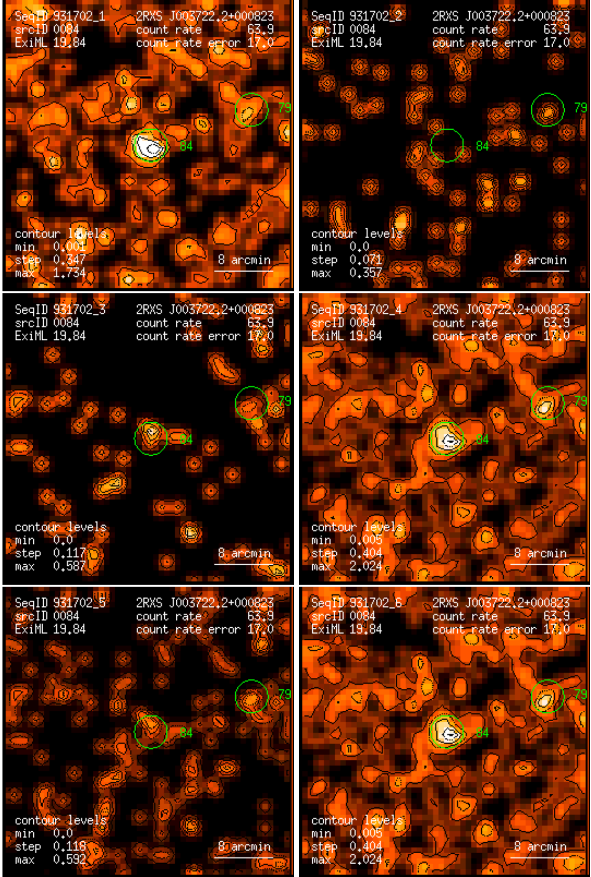
Figure 84: RASS 931702: detection 0084: band rate images, Gaussian filter: (1) PSPC channels 11 – 41, (2) 52 – 90, (3) 91 – 201, (4) 11 – 235, (5) 52 – 201, (6) 11 – 201. Broad band rates in counts/ks. Band rate contour levels in counts/ks/arcmin 2 .
