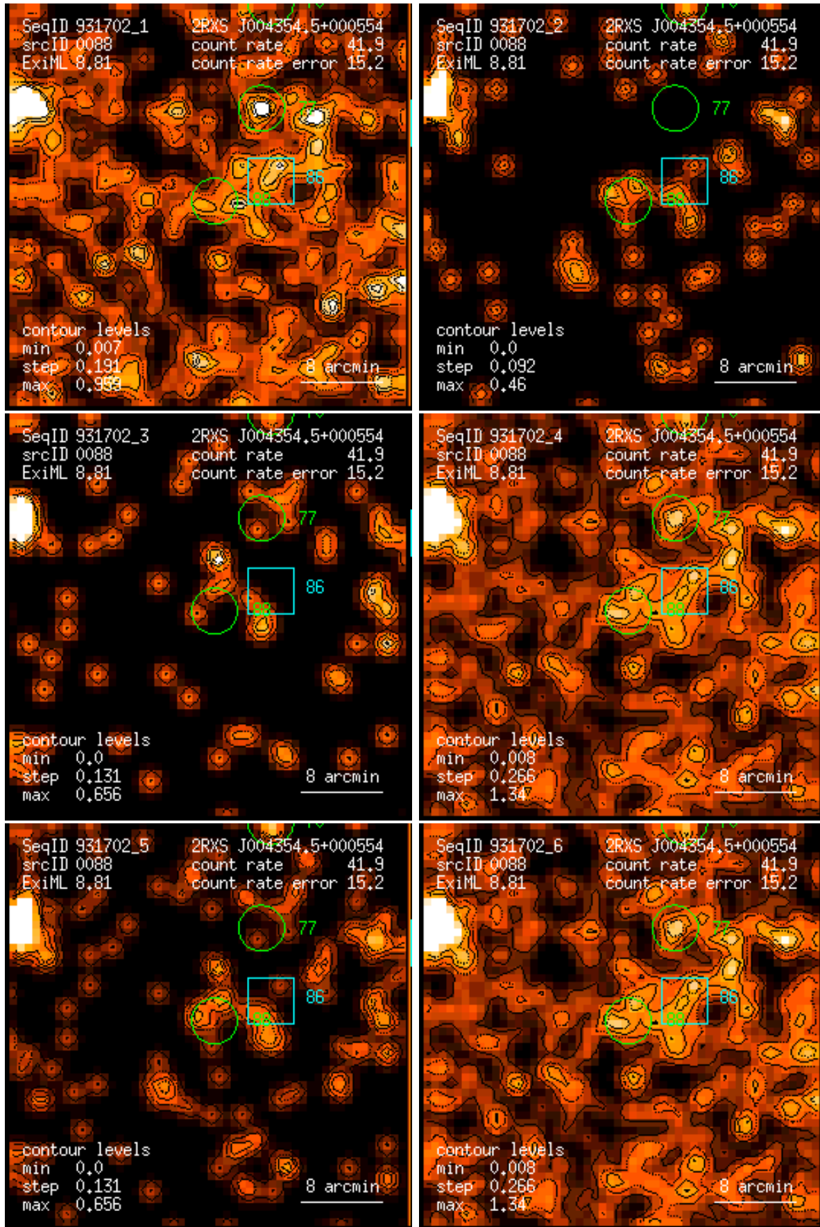
Figure 88: RASS 931702: detection 0088: band rate images, Gaussian filter: (1) PSPC channels 11 – 41, (2) 52 – 90, (3) 91 – 201, (4) 11 – 235, (5) 52 – 201, (6) 11 – 201. Broad band rates in counts/ks. Band rate contour levels in counts/ks/arcmin 2 .
