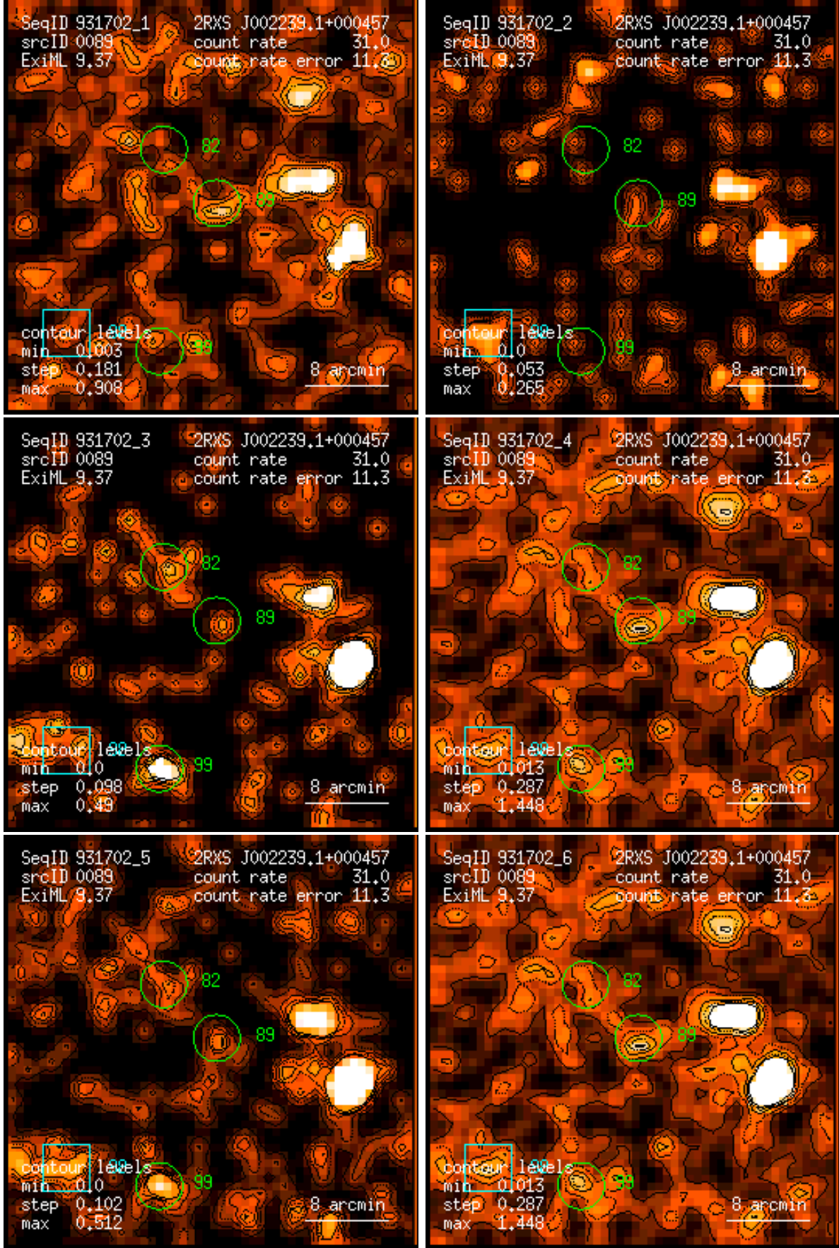
Figure 89: RASS 931702: detection 0089: band rate images, Gaussian filter: (1) PSPC channels 11 – 41, (2) 52 – 90, (3) 91 – 201, (4) 11 – 235, (5) 52 – 201, (6) 11 – 201. Broad band rates in counts/ks. Band rate contour levels in counts/ks/arcmin 2 .
