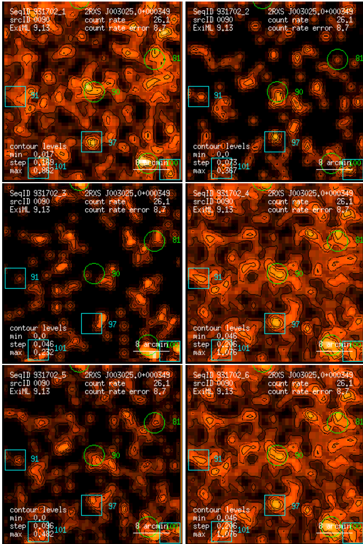
Figure 90: RASS 931702: detection 0090: band rate images, Gaussian filter: (1) PSPC channels 11 – 41, (2) 52 – 90, (3) 91 – 201, (4) 11 – 235, (5) 52 – 201, (6) 11 – 201. Broad band rates in counts/ks. Band rate contour levels in counts/ks/arcmin 2 .
