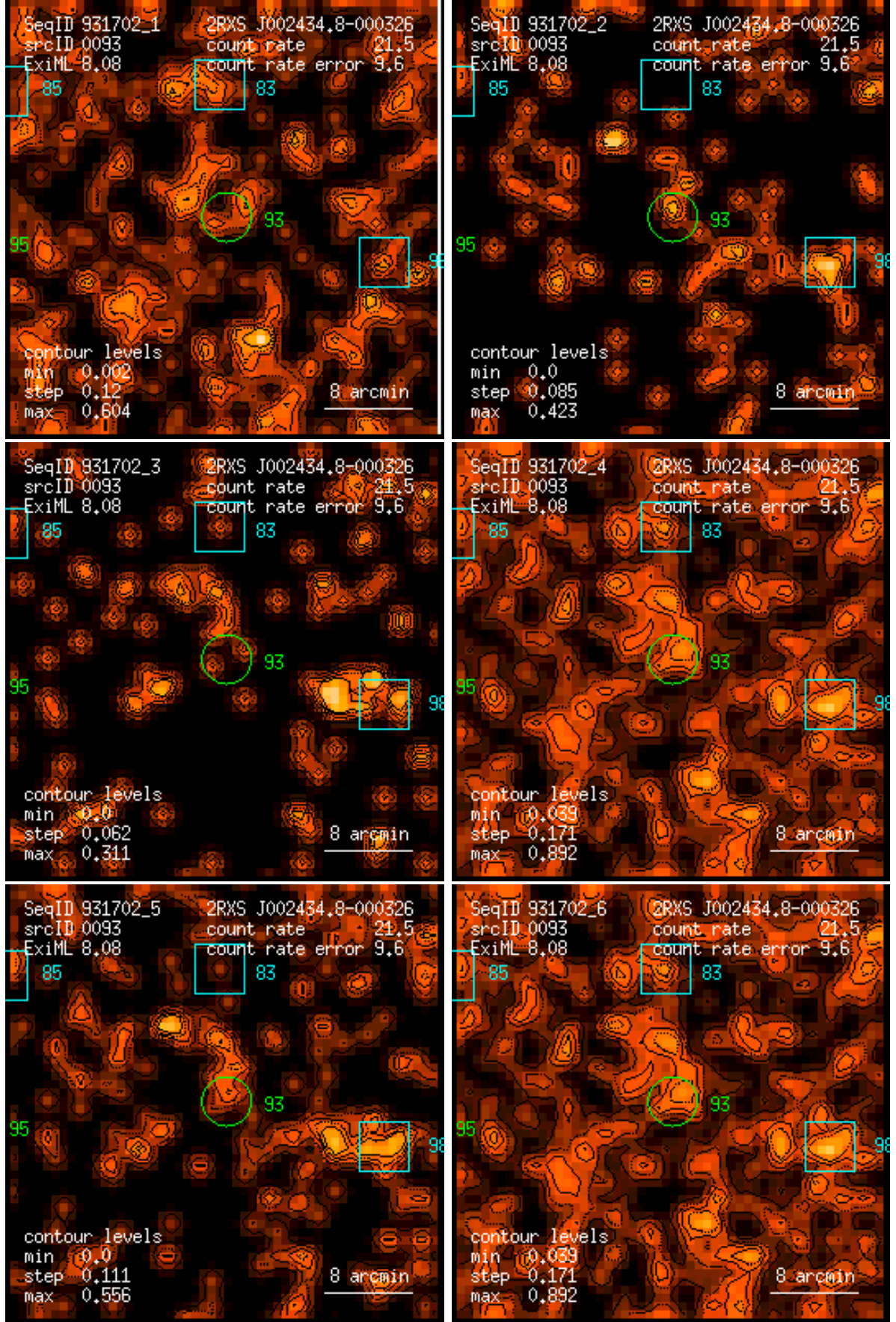
Figure 93: RASS 931702: detection 0093: band rate images, Gaussian filter: (1) PSPC channels 11 – 41, (2) 52 – 90, (3) 91 – 201, (4) 11 – 235, (5) 52 – 201, (6) 11 – 201. Broad band rates in counts/ks. Band rate contour levels in counts/ks/arcmin 2 .
