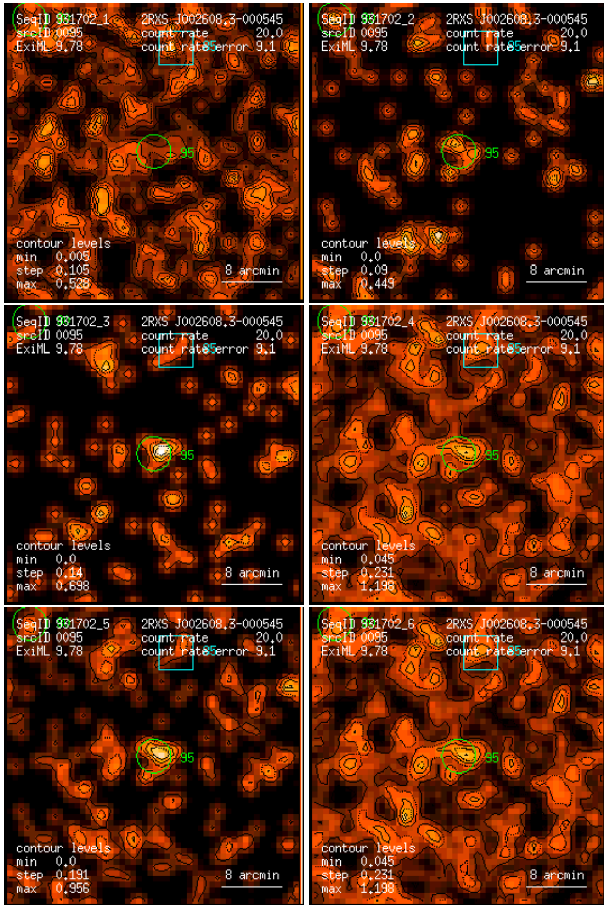
Figure 95: RASS 931702: detection 0095: band rate images, Gaussian filter: (1) PSPC channels 11 – 41, (2) 52 – 90, (3) 91 – 201, (4) 11 – 235, (5) 52 – 201, (6) 11 – 201. Broad band rates in counts/ks. Band rate contour levels in counts/ks/arcmin 2 .
