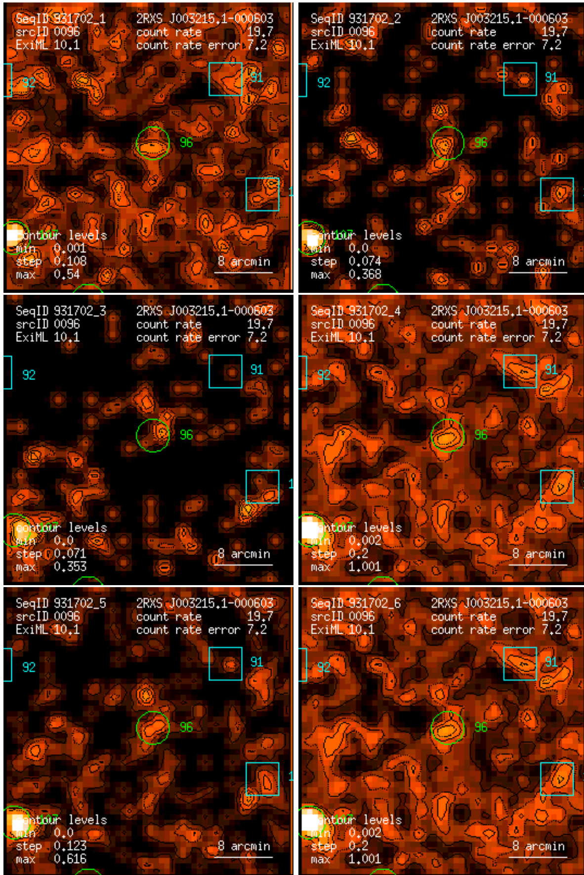
Figure 96: RASS 931702: detection 0096: band rate images, Gaussian filter: (1) PSPC channels 11 – 41, (2) 52 – 90, (3) 91 – 201, (4) 11 – 235, (5) 52 – 201, (6) 11 – 201. Broad band rates in counts/ks. Band rate contour levels in counts/ks/arcmin 2 .
