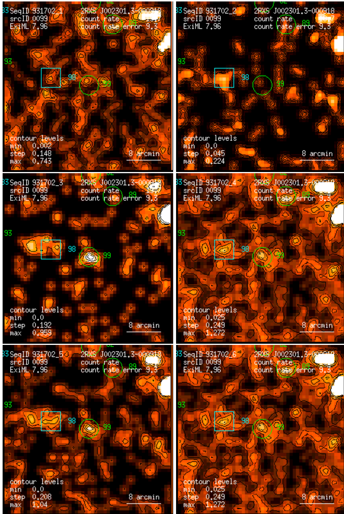
Figure 99: RASS 931702: detection 0099: band rate images, Gaussian filter: (1) PSPC channels 11 – 41, (2) 52 – 90, (3) 91 – 201, (4) 11 – 235, (5) 52 – 201, (6) 11 – 201. Broad band rates in counts/ks. Band rate contour levels in counts/ks/arcmin 2 .
