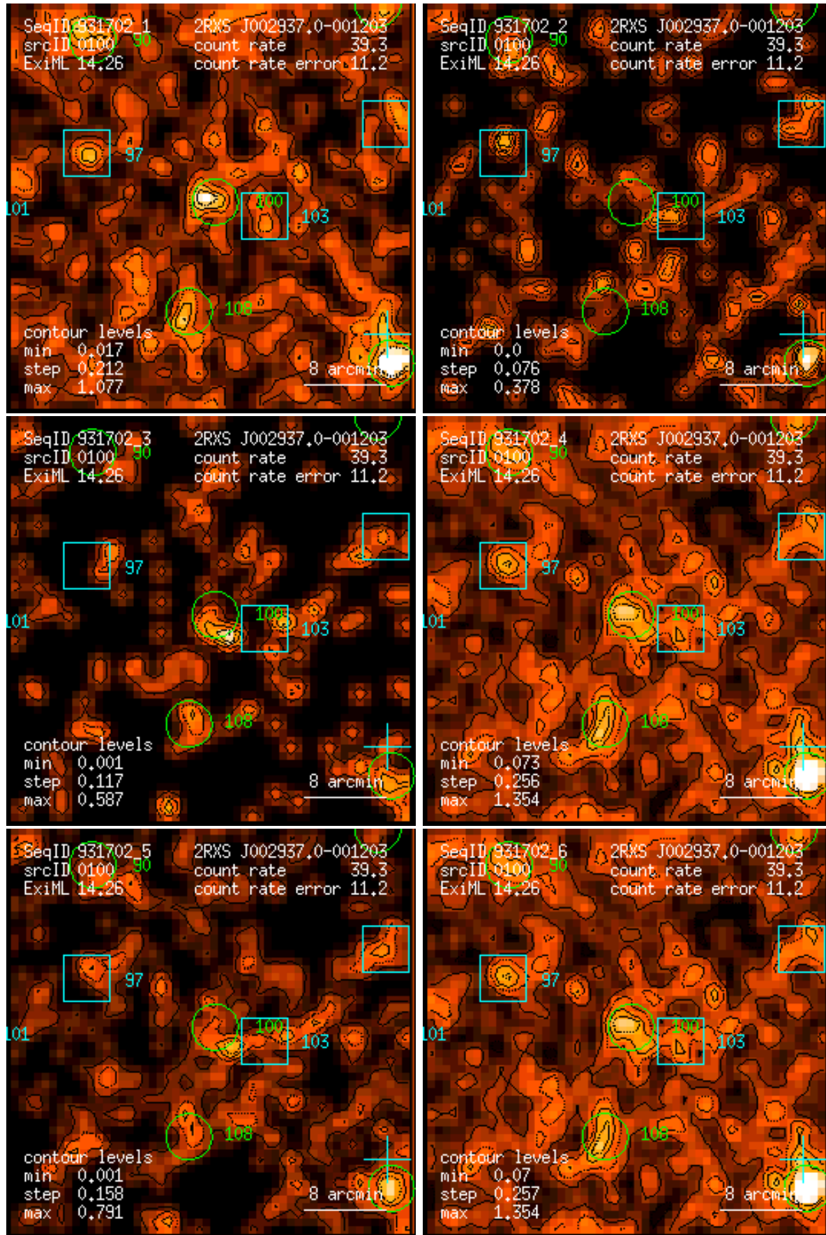
Figure 100: RASS 931702: detection 0100: band rate images, Gaussian filter: (1) PSPC channels 11 – 41, (2) 52 – 90, (3) 91 – 201, (4) 11 – 235, (5) 52 – 201, (6) 11 – 201. Broad band rates in counts/ks. Band rate contour levels in counts/ks/arcmin 2 .
