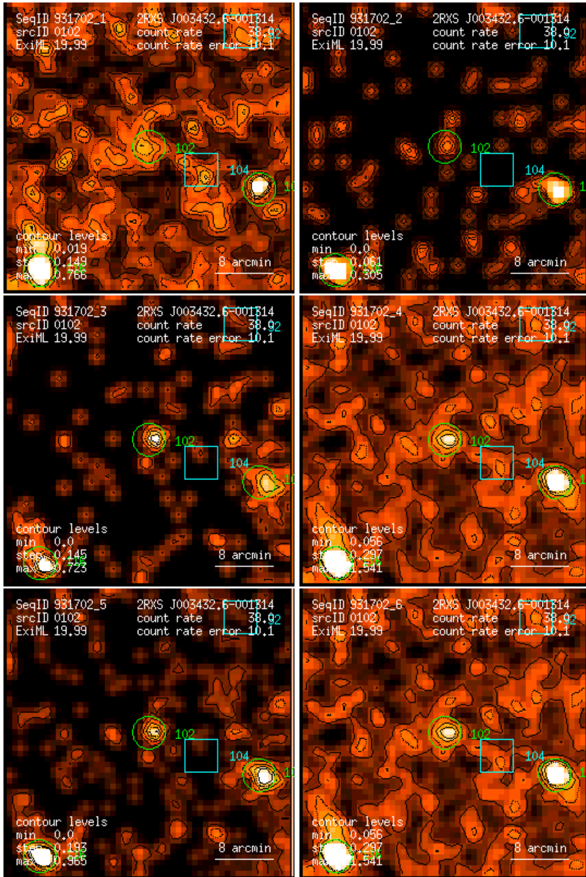
Figure 102: RASS 931702: detection 0102: band rate images, Gaussian filter: (1) PSPC channels 11 – 41, (2) 52 – 90, (3) 91 – 201, (4) 11 – 235, (5) 52 – 201, (6) 11 – 201. Broad band rates in counts/ks. Band rate contour levels in counts/ks/arcmin 2 .
