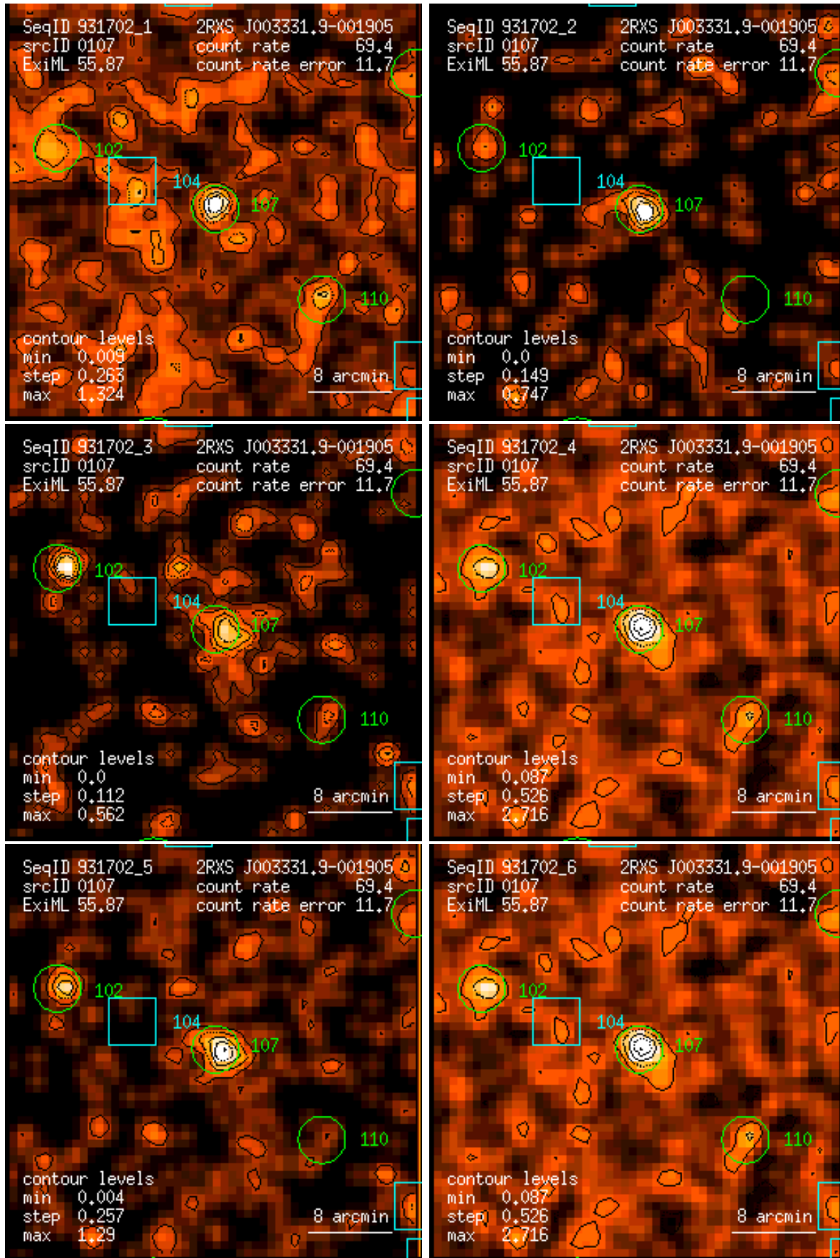
Figure 107: RASS 931702: detection 0107: band rate images, Gaussian filter: (1) PSPC channels 11 – 41, (2) 52 – 90, (3) 91 – 201, (4) 11 – 235, (5) 52 – 201, (6) 11 – 201. Broad band rates in counts/ks. Band rate contour levels in counts/ks/arcmin 2 .
