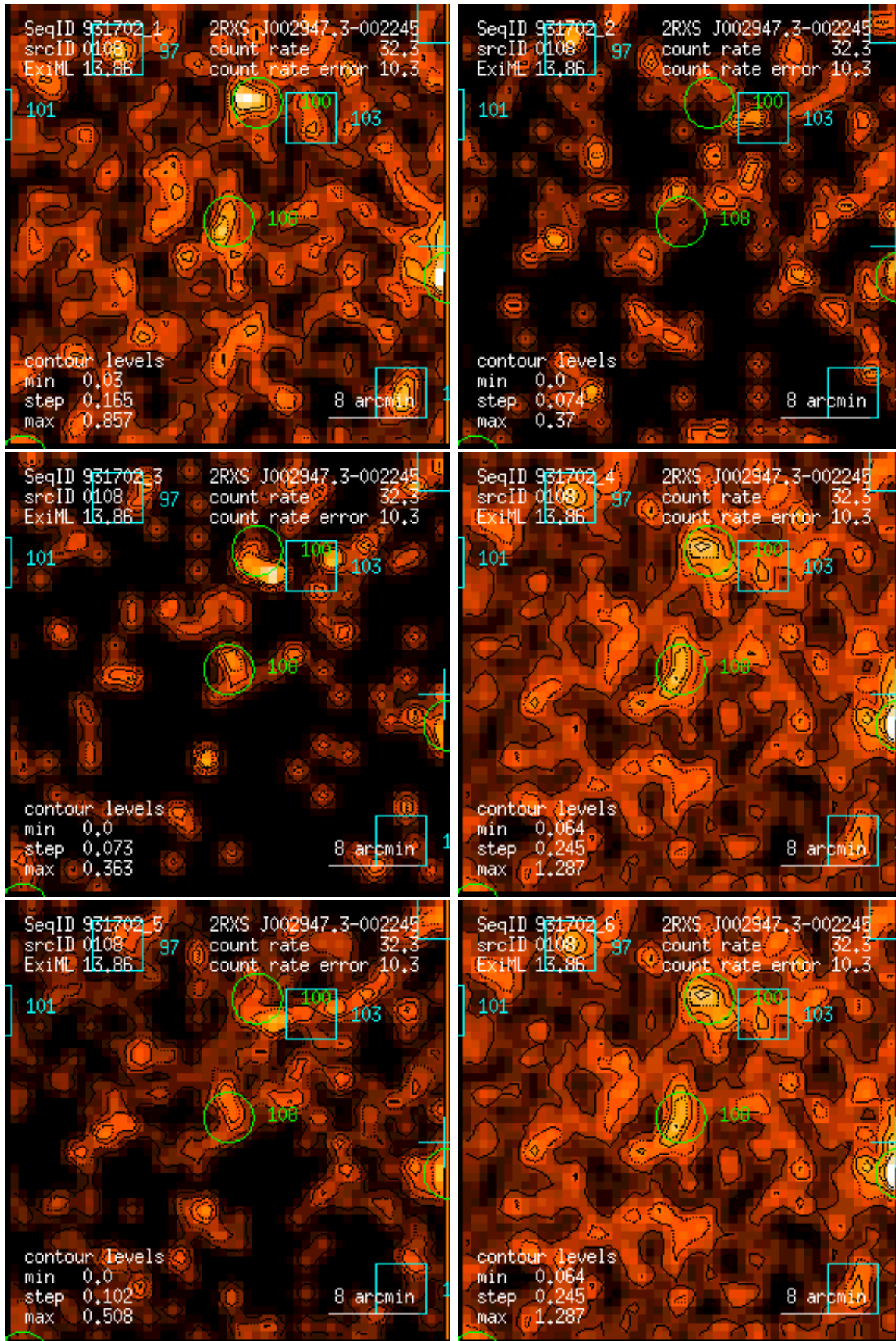
Figure 108: RASS 931702: detection 0108: band rate images, Gaussian filter: (1) PSPC channels 11 – 41, (2) 52 – 90, (3) 91 – 201, (4) 11 – 235, (5) 52 – 201, (6) 11 – 201. Broad band rates in counts/ks. Band rate contour levels in counts/ks/arcmin 2 .
