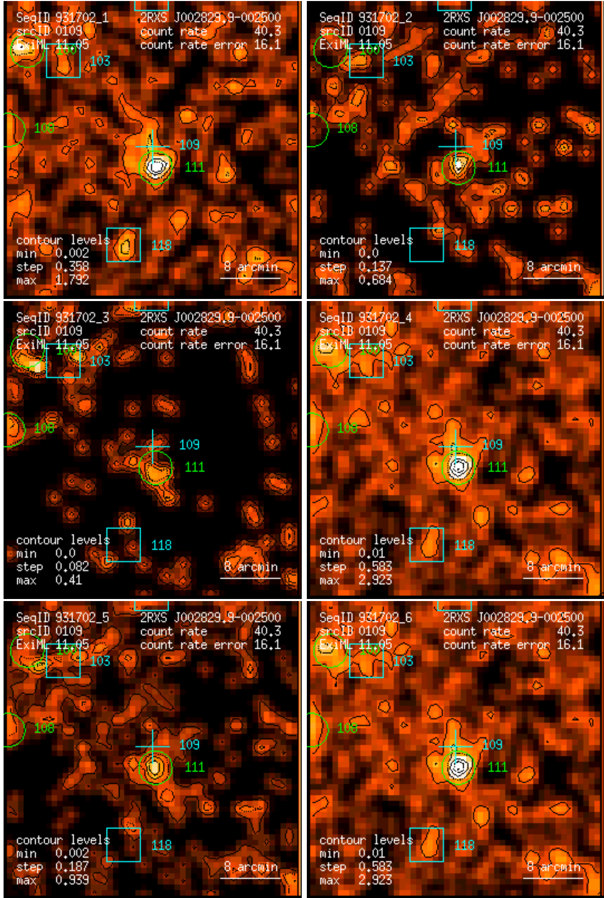
Figure 109: RASS 931702: detection 0109: band rate images, Gaussian filter: (1) PSPC channels 11 – 41, (2) 52 – 90, (3) 91 – 201, (4) 11 – 235, (5) 52 – 201, (6) 11 – 201. Broad band rates in counts/ks. Band rate contour levels in counts/ks/arcmin 2 .
