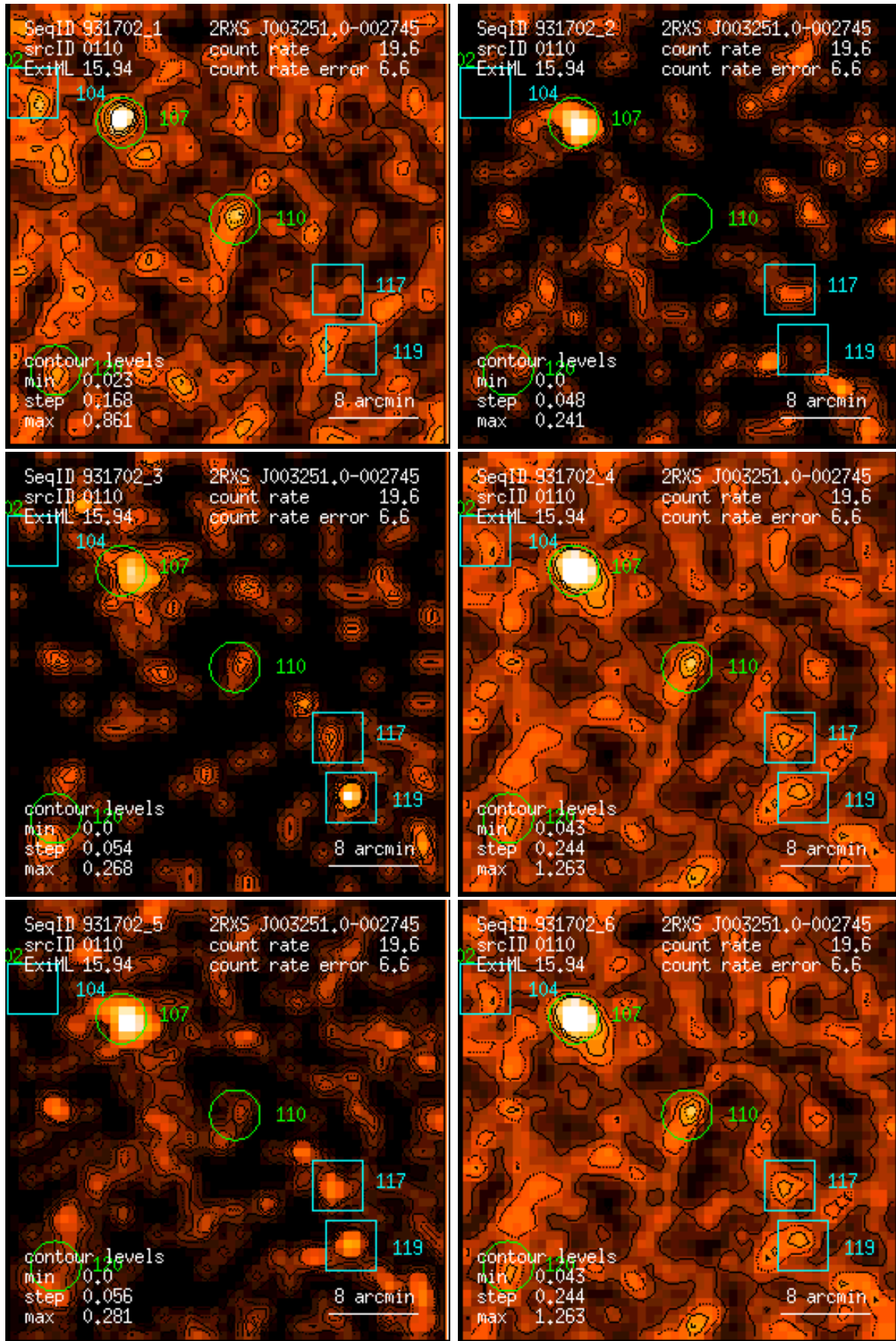
Figure 110: RASS 931702: detection 0110: band rate images, Gaussian filter: (1) PSPC channels 11 – 41, (2) 52 – 90, (3) 91 – 201, (4) 11 – 235, (5) 52 – 201, (6) 11 – 201. Broad band rates in counts/ks. Band rate contour levels in counts/ks/arcmin 2 .
