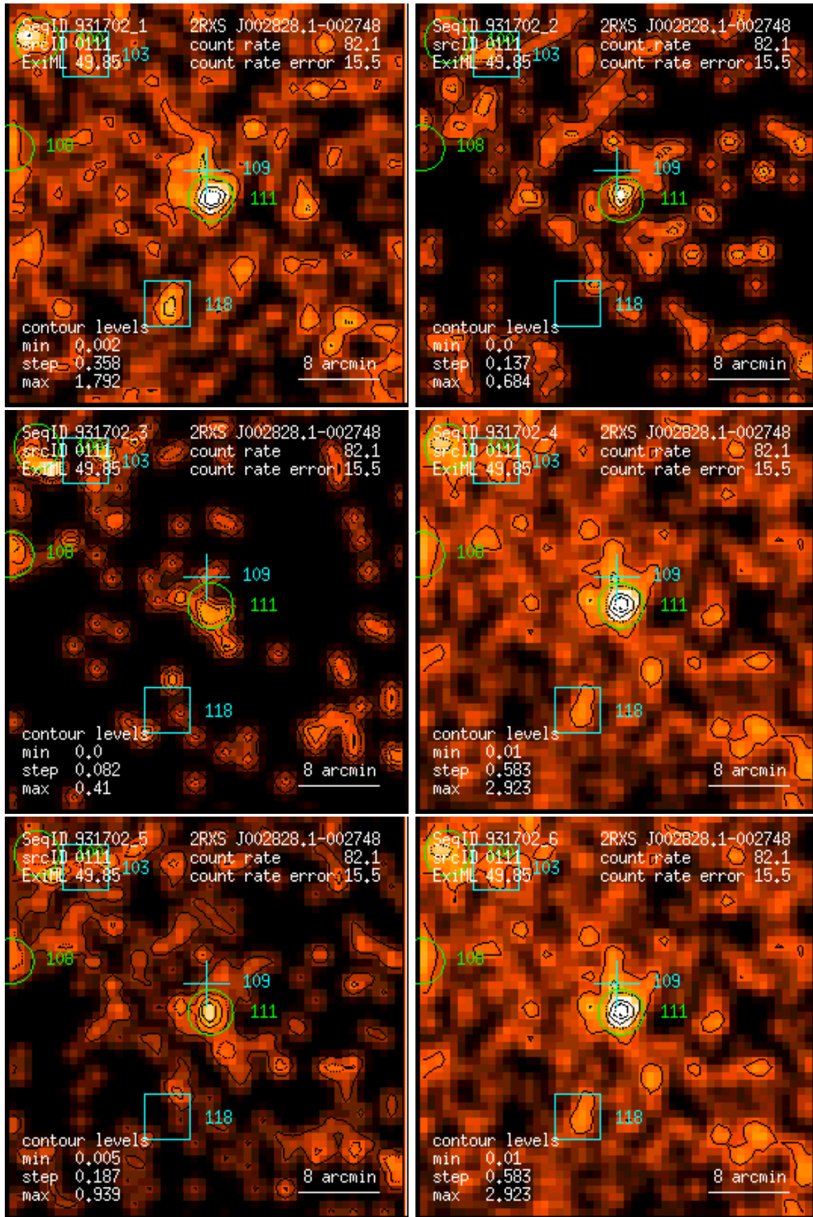
Figure 111: RASS 931702: detection 0111: band rate images, Gaussian filter: (1) PSPC channels 11 – 41, (2) 52 – 90, (3) 91 – 201, (4) 11 – 235, (5) 52 – 201, (6) 11 – 201. Broad band rates in counts/ks. Band rate contour levels in counts/ks/arcmin 2 .
