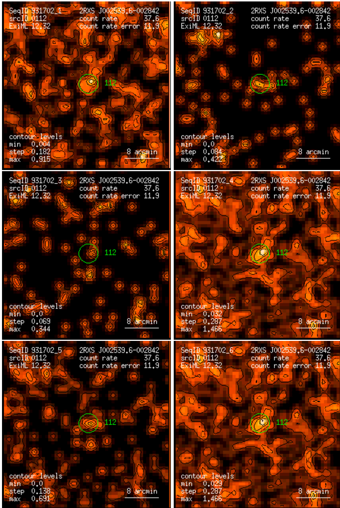
Figure 112: RASS 931702: detection 0112: band rate images, Gaussian filter: (1) PSPC channels 11 – 41, (2) 52 – 90, (3) 91 – 201, (4) 11 – 235, (5) 52 – 201, (6) 11 – 201. Broad band rates in counts/ks. Band rate contour levels in counts/ks/arcmin 2 .
