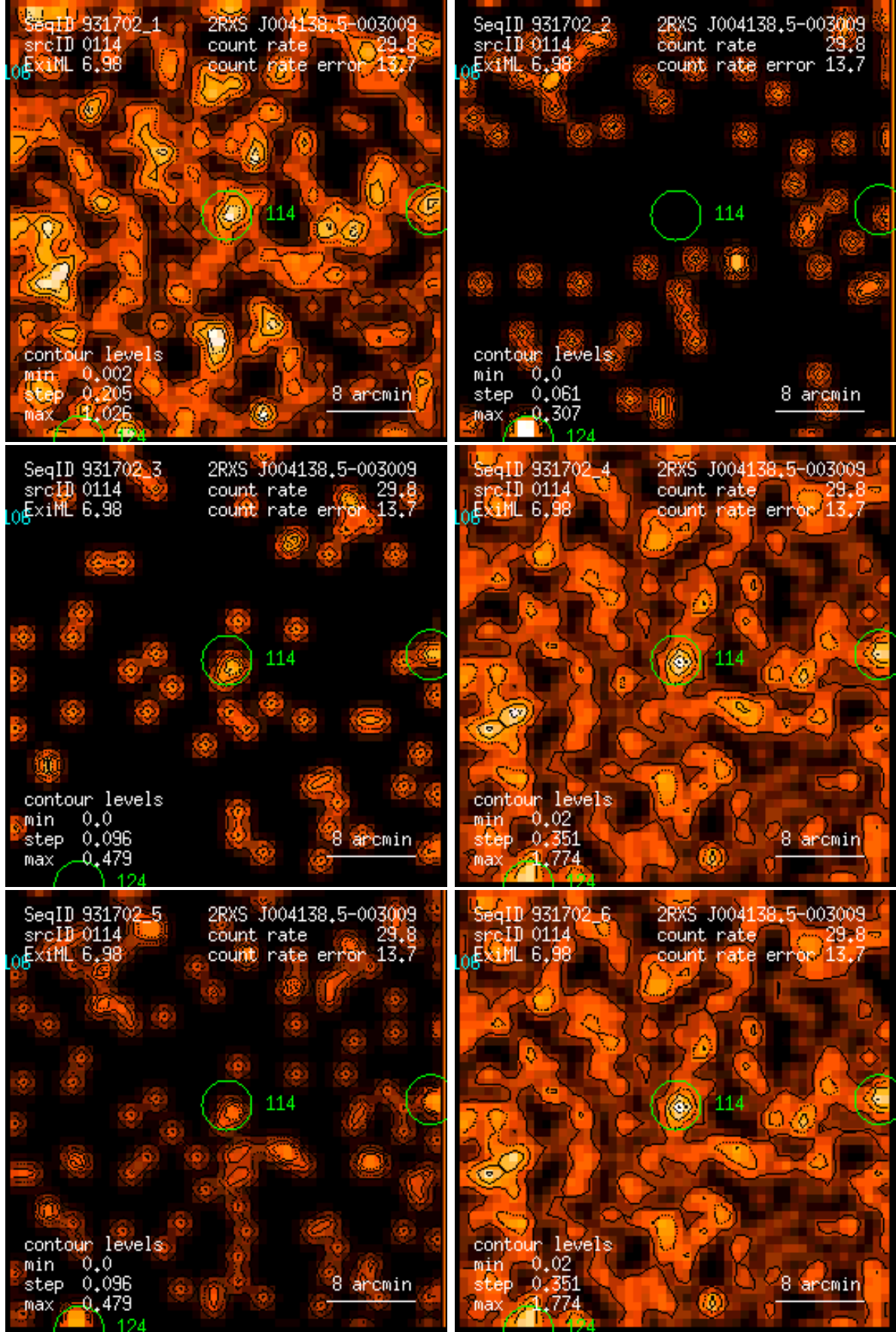
Figure 114: RASS 931702: detection 0114: band rate images, Gaussian filter: (1) PSPC channels 11 – 41, (2) 52 – 90, (3) 91 – 201, (4) 11 – 235, (5) 52 – 201, (6) 11 – 201. Broad band rates in counts/ks. Band rate contour levels in counts/ks/arcmin 2 .
