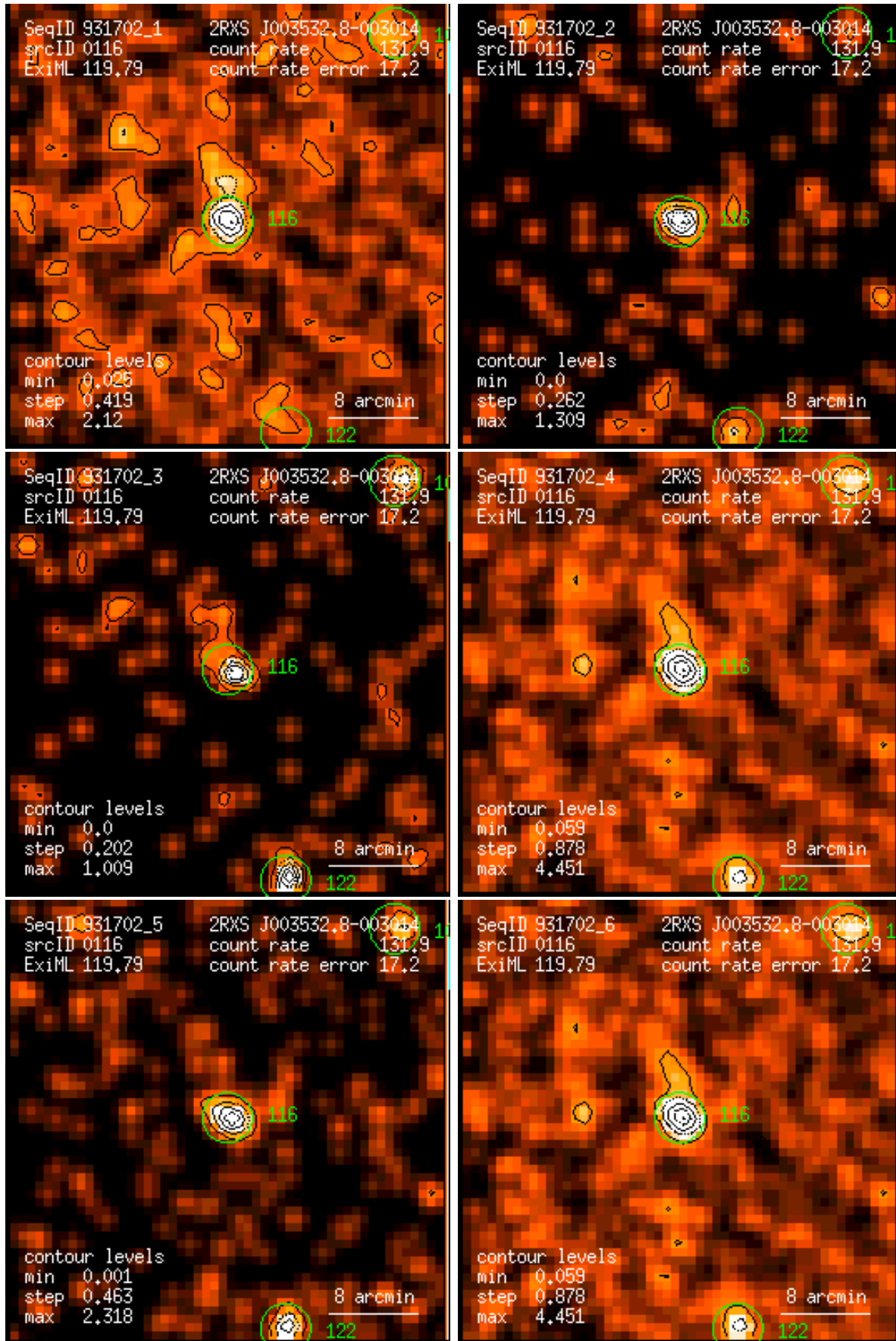
Figure 116: RASS 931702: detection 0116: band rate images, Gaussian filter: (1) PSPC channels 11 – 41, (2) 52 – 90, (3) 91 – 201, (4) 11 – 235, (5) 52 – 201, (6) 11 – 201. Broad band rates in counts/ks. Band rate contour levels in counts/ks/arcmin 2 .
