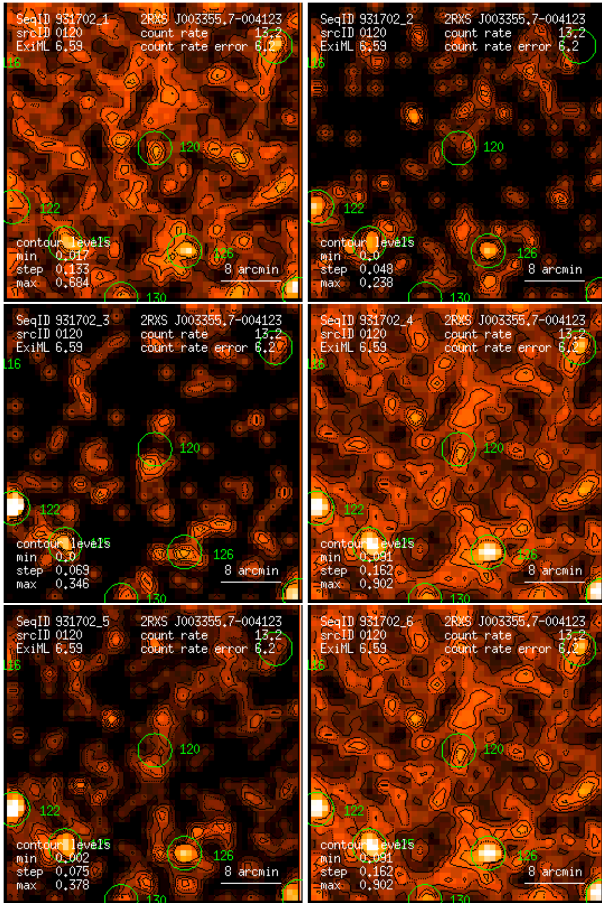
Figure 120: RASS 931702: detection 0120: band rate images, Gaussian filter: (1) PSPC channels 11 – 41, (2) 52 – 90, (3) 91 – 201, (4) 11 – 235, (5) 52 – 201, (6) 11 – 201. Broad band rates in counts/ks. Band rate contour levels in counts/ks/arcmin 2 .
