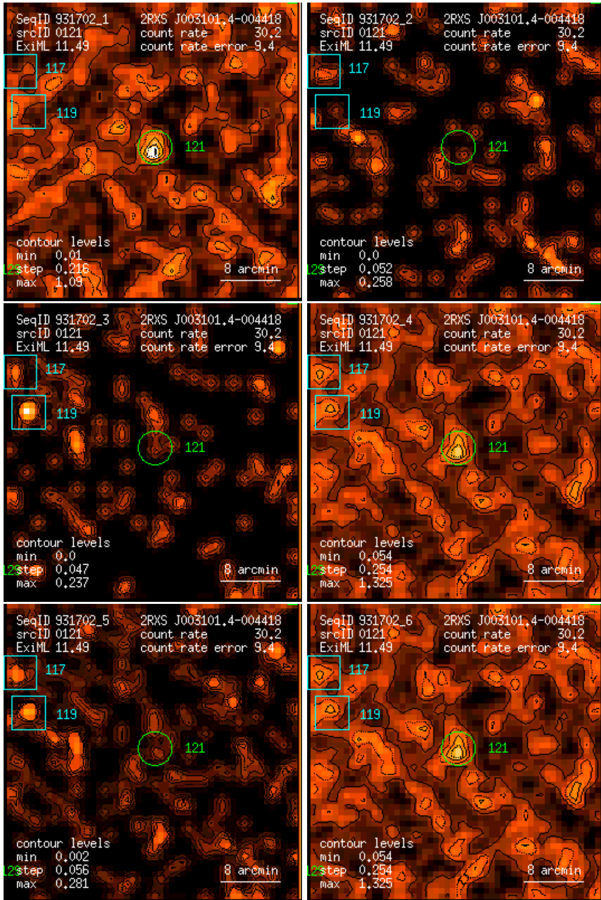
Figure 121: RASS 931702: detection 0121: band rate images, Gaussian filter: (1) PSPC channels 11 – 41, (2) 52 – 90, (3) 91 – 201, (4) 11 – 235, (5) 52 – 201, (6) 11 – 201. Broad band rates in counts/ks. Band rate contour levels in counts/ks/arcmin 2 .
