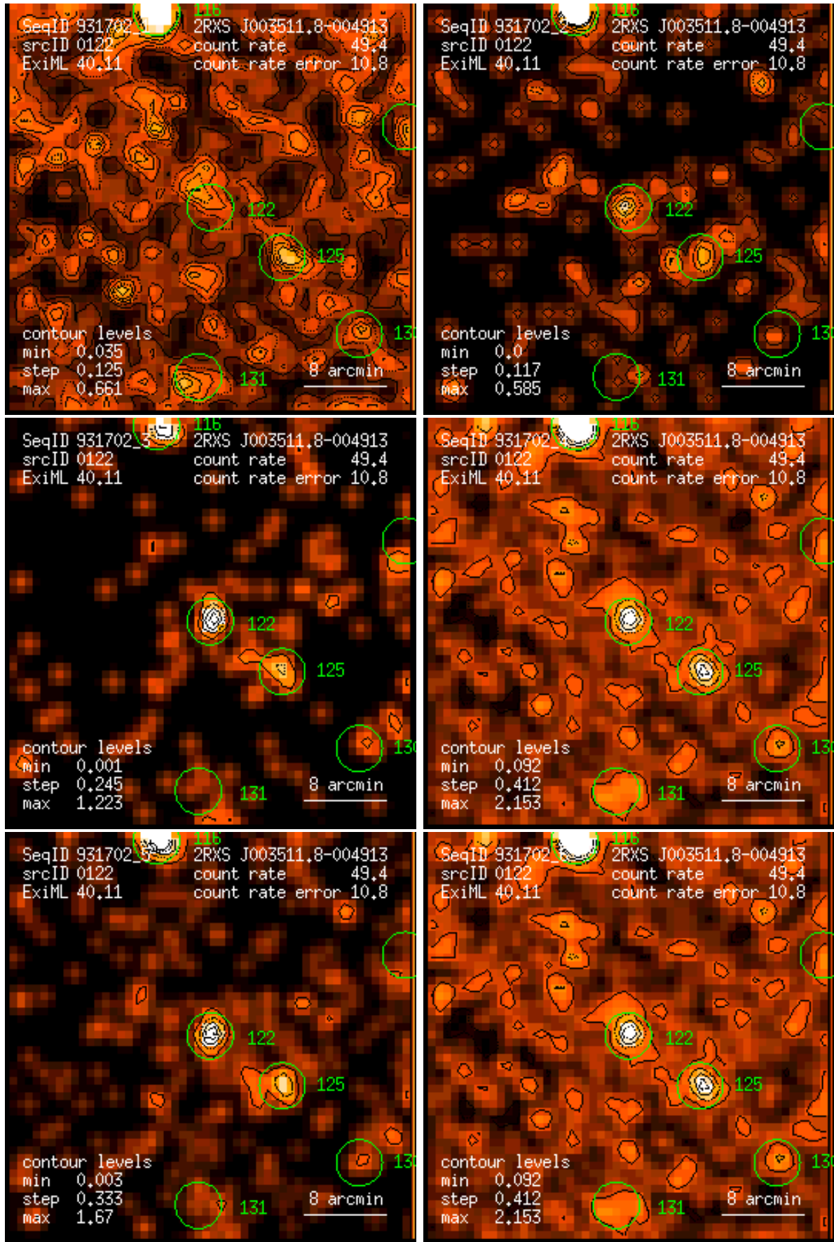
Figure 122: RASS 931702: detection 0122: band rate images, Gaussian filter: (1) PSPC channels 11 – 41, (2) 52 – 90, (3) 91 – 201, (4) 11 – 235, (5) 52 – 201, (6) 11 – 201. Broad band rates in counts/ks. Band rate contour levels in counts/ks/arcmin 2 .
