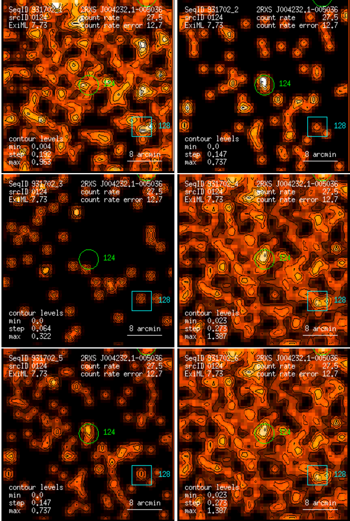
Figure 124: RASS 931702: detection 0124: band rate images, Gaussian filter: (1) PSPC channels 11 – 41, (2) 52 – 90, (3) 91 – 201, (4) 11 – 235, (5) 52 – 201, (6) 11 – 201. Broad band rates in counts/ks. Band rate contour levels in counts/ks/arcmin 2 .
