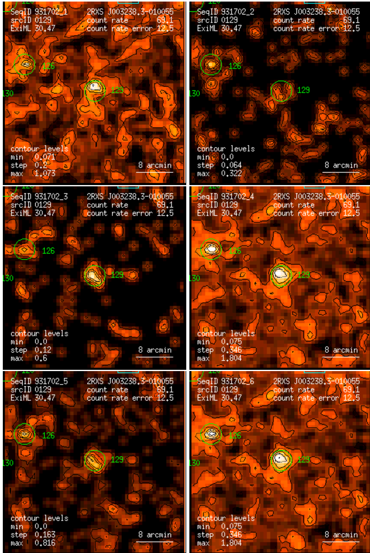
Figure 129: RASS 931702: detection 0129: band rate images, Gaussian filter: (1) PSPC channels 11 – 41, (2) 52 – 90, (3) 91 – 201, (4) 11 – 235, (5) 52 – 201, (6) 11 – 201. Broad band rates in counts/ks. Band rate contour levels in counts/ks/arcmin 2 .
