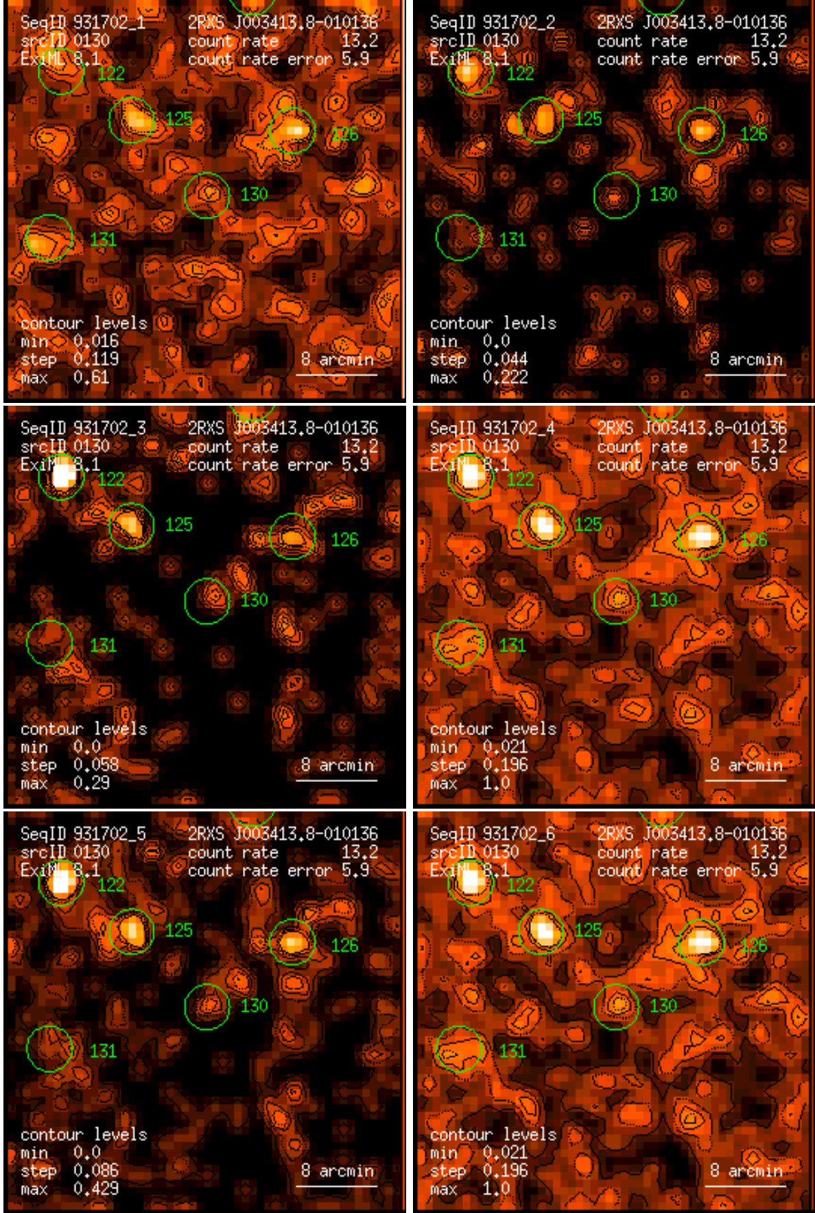
Figure 130: RASS 931702: detection 0130: band rate images, Gaussian filter: (1) PSPC channels 11 – 41, (2) 52 – 90, (3) 91 – 201, (4) 11 – 235, (5) 52 – 201, (6) 11 – 201. Broad band rates in counts/ks. Band rate contour levels in counts/ks/arcmin 2 .
