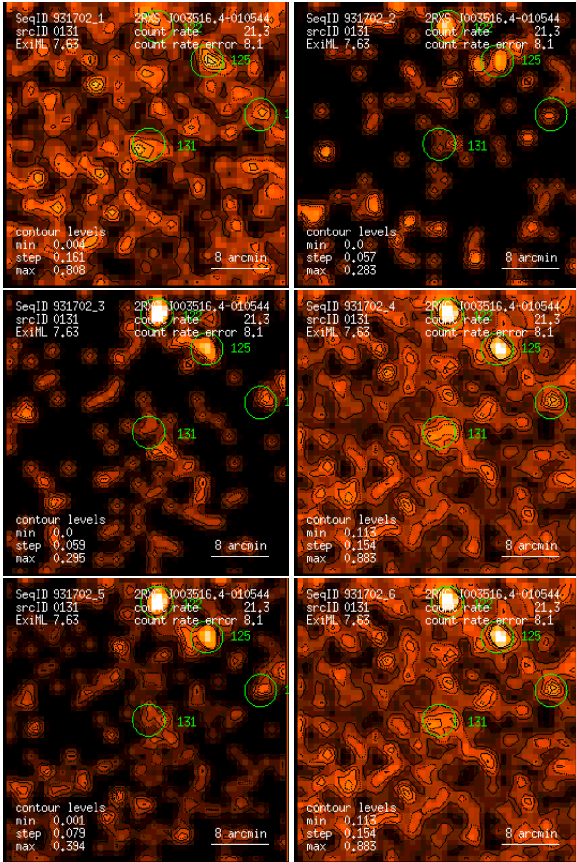
Figure 131: RASS 931702: detection 0131: band rate images, Gaussian filter: (1) PSPC channels 11 – 41, (2) 52 – 90, (3) 91 – 201, (4) 11 – 235, (5) 52 – 201, (6) 11 – 201. Broad band rates in counts/ks. Band rate contour levels in counts/ks/arcmin 2 .
